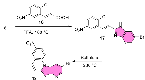
Sch. (2). Synthesis of a complex imidazo[4,5- b ] pyridine.
