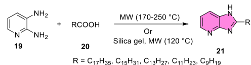
Sch. (3). Synthetic of imidazo[4,5- b ] pyridine by microwave energy.
