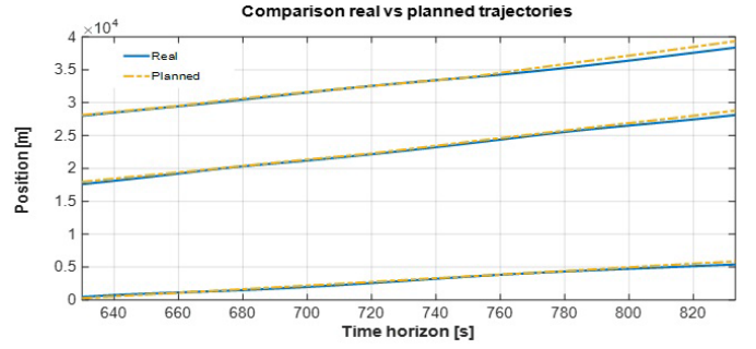
Fig. 14. Trend for the real and planned values of the states for the three trains (scenario III). The full lines display the real trajectories while dashed lines represent the planned ones.
