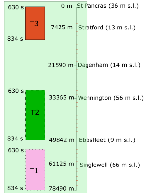
Fig. 5. Track topography on which validation has been achieved. In the time interval 630 - 834 s the three trains T1,T2,T3 are planned to cover a space shown by the related rectangles.
