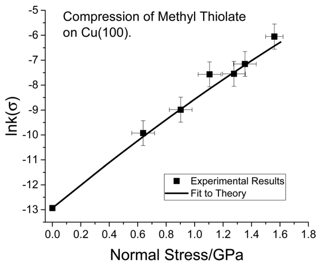
Fig. 3 Plot of the logarithm of rate of the normal-stress-induced decomposition of methyl thiolate on Cu(100) as a function of the normal stress in GPa (■) 1 compared with the theoretical plot from eqn (3) using parameters derived from the data in Fig. 2, so that the plot requires no adjustable parameters.
