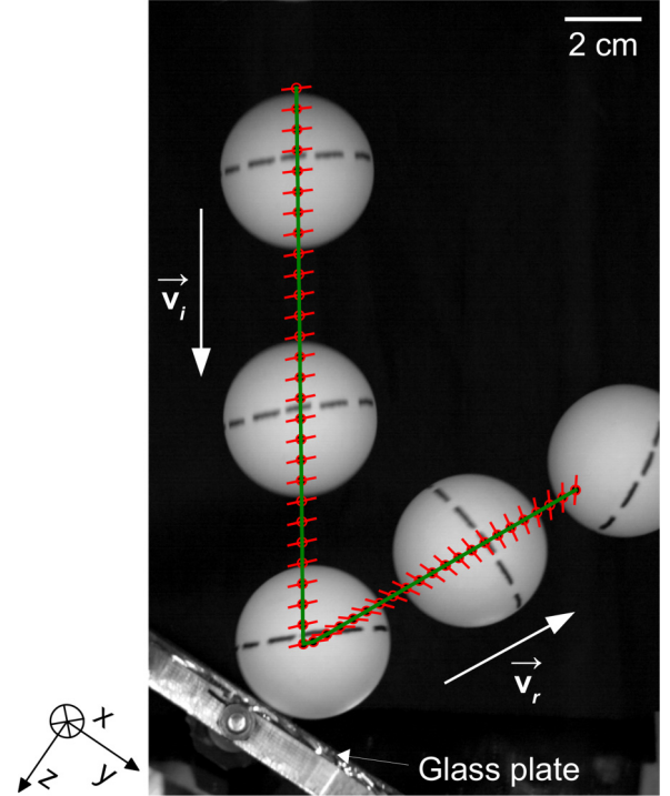
FIG. 2. Superimposition of five images of the ball around the collision with the tilted glass window and associated trajectory. Only five images separated by a time difference of 5.6 ms are displayed here. The black dashed line drawn on the ball allows identifying the ball joint and is used for the determination of the ball angular velocity. For each image of the movie (frame rate: 2142 fps), we determine the position of the center of the ball (red circle) and the angular position of the ball (red dashed). From the successive positions of the center we obtain the incidence angle \theta_i = 35^\circ and the incident velocity v_i = 11.6 m s -1 . From the successive angular positions of the ball we get the angular velocity \omega_r = 190 rad s -1 .
