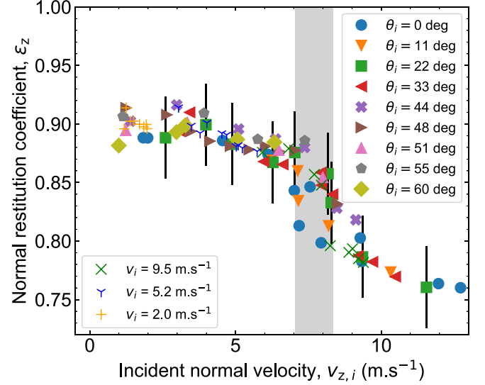
FIG. 4. Restitution coefficient of normal velocity \varepsilon_z vs normal velocity v_{z,i} . The collapse of the data in a single trend shows that the restitution of the normal component of the velocity is not altered by the tangential component. The gray vertical region highlights the transition to the buckling instability which occurs within the vicinity of the critical velocity v_{z,i}^c = (7.5 \pm 0.5) \text{ m s}^{-1} .
