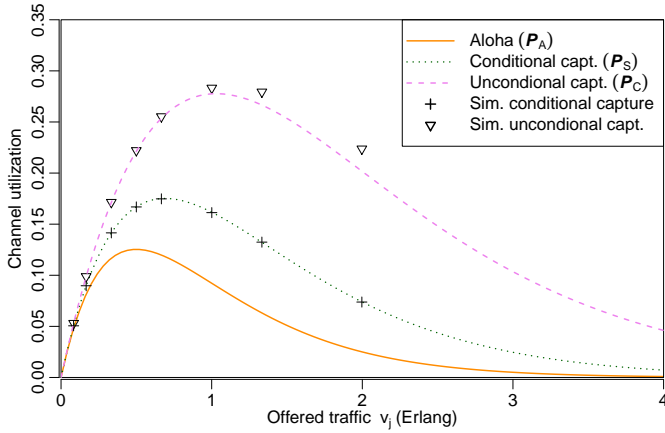
Figure 3. Channel utilization as a function of load for three PDR models with all nodes at 7.5 km from the gateway, and comparison with simulation results (+ and \nabla ). For P_C , reception is subject to dominating the sum of interference by factor \xi = 1 dB. The model slightly underestimates PDR when the load is high, beyond maximal channel utilization.
