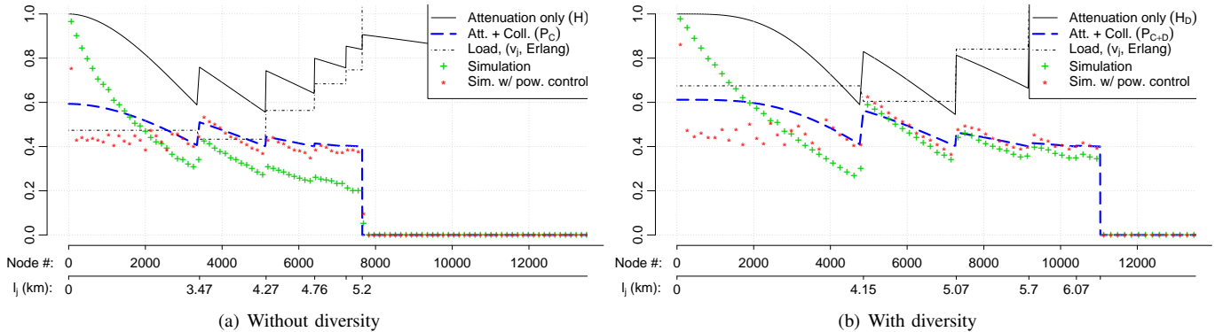
Figure 12. Packet delivery ratio with inter-SF interference, SF allocation targeting PDR of at least 0.4, high node density of 90 nodes per \text{km}^2 . + : simulation without power control, * : simulation with power control in the SF7 zone. Power control is very effective to obviate the impact of imperfect orthogonality.
