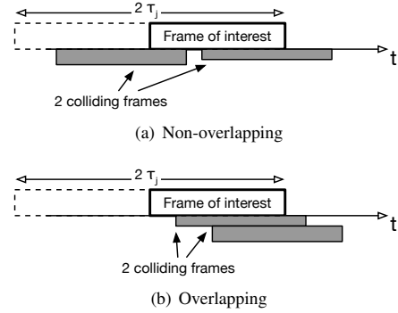
Figure 1. Collision with two other frames: overlapping and non-overlapping scenarios
