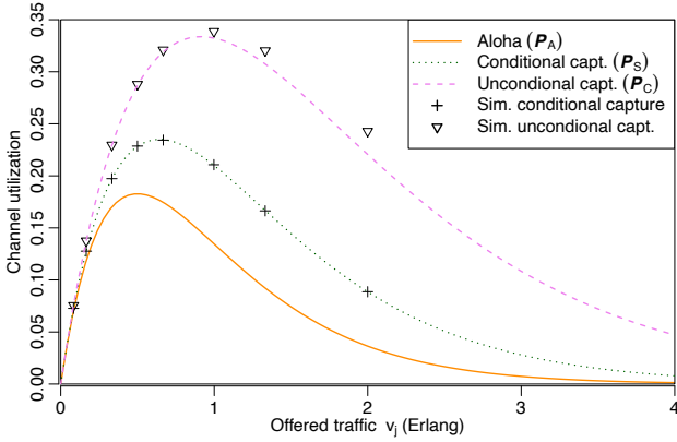
Figure 2. Channel utilization as a function of load for three PDR models with all nodes at 2.5 km from the gateway and comparison with simulation. For P_C , reception is subject to dominating the sum of interference by factor \xi = 1 dB. For high load, the approximation of overlapping frames for n > 2 causes the model to underestimate PDR , compared to the result obtained by simulation ( \nabla ). Compared to ALOHA ( P_A ) or reception subject to finding an empty channel ( P_S , simulations: + ) [20], maximal utilization is much higher and for a higher load.
