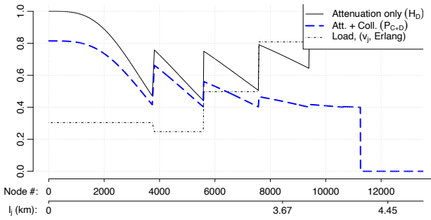
Figure 11. Adding SF6, for high node density and with diversity; the capacity gain is limited
