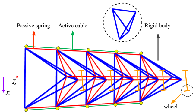
Fig. 1. A tensegrity robotic snake.
