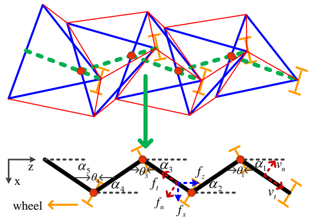
Fig. 2. A simplified diagram of the tensegrity robotic snake.
