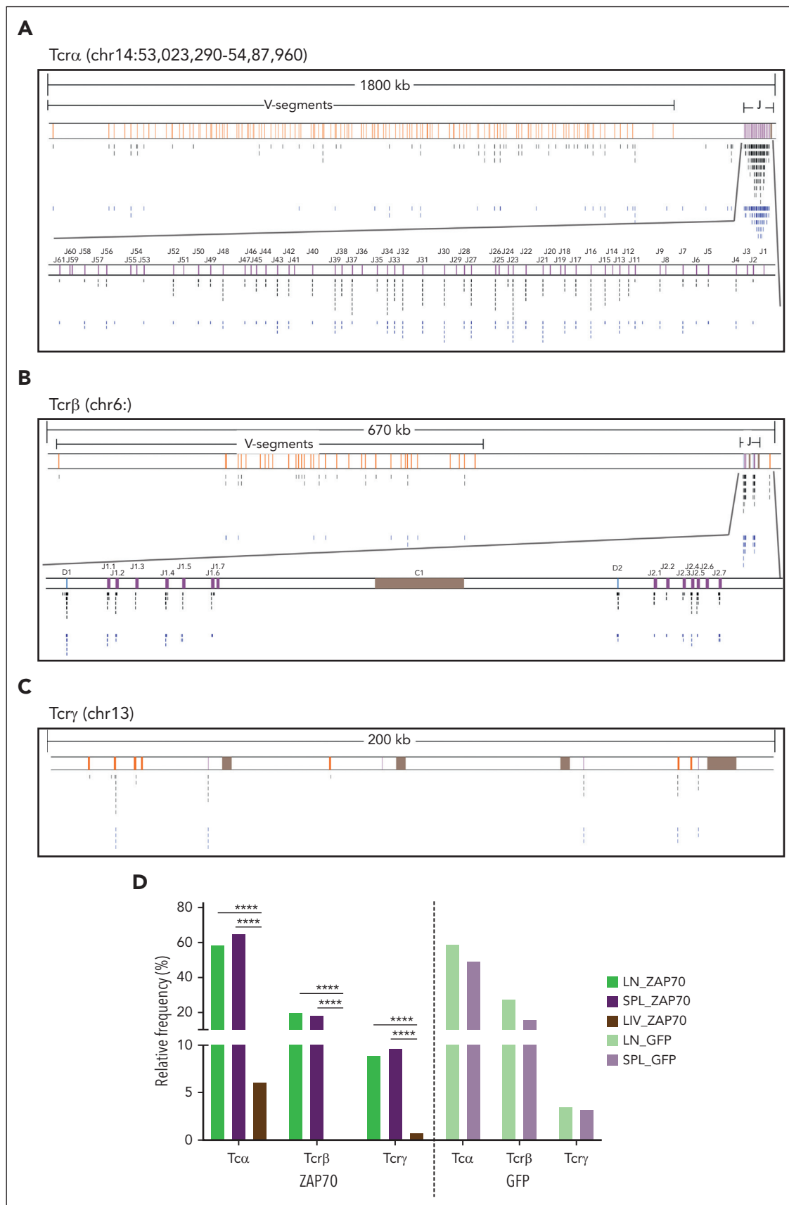
Figure 3. Distribution of AAV ISs within Tcr loci. (A-C) Genomic distribution of AAV IS in the LN and SPL data sets of ZAP70-treated mice and targeting TCR genes: TCR \alpha (A), TCR \beta (B), and TCR \gamma (C), as indicated. Genomic coordinates and scale are indicated in each panel. Black and blue lines indicate the position of the AAV IS from the LN (black) and SPL (blue) data sets. V, D, and J segments are indicated by yellow, blue, and purple rectangles, respectively. (C) Constant regions are represented as brown
