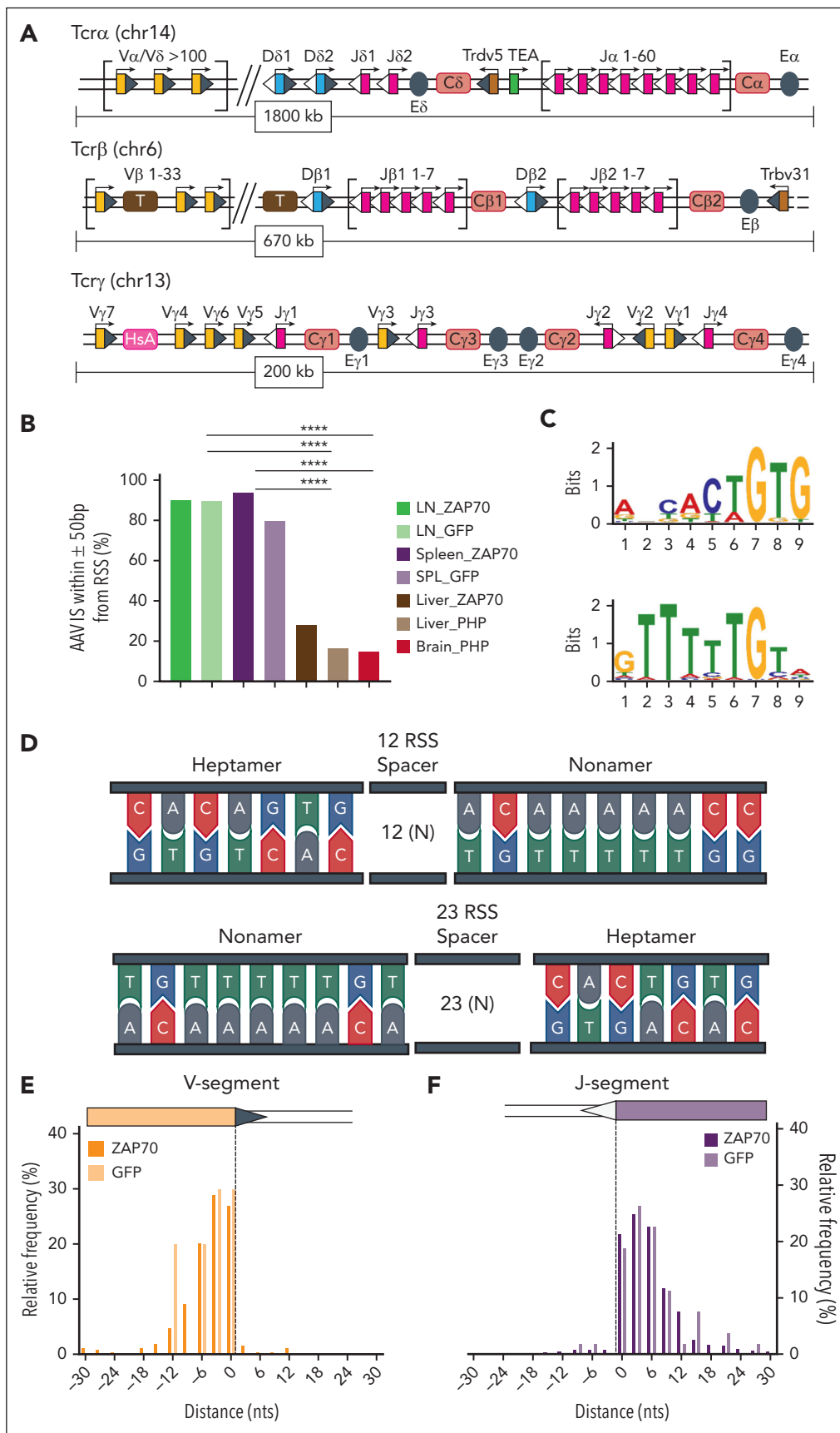
Figure 4. AAV integrations occurred at RAG-induced DSBs. (A) Schematic representation of the organization of the murine Tcrα / Tcrδ , Tcry , and Tcrβ loci. Genomic proportions are not preserved. V, D, and J segments are indicated by yellow, blue, and purple rectangles, respectively. RSS are represented as triangles close to the V, D, and J
