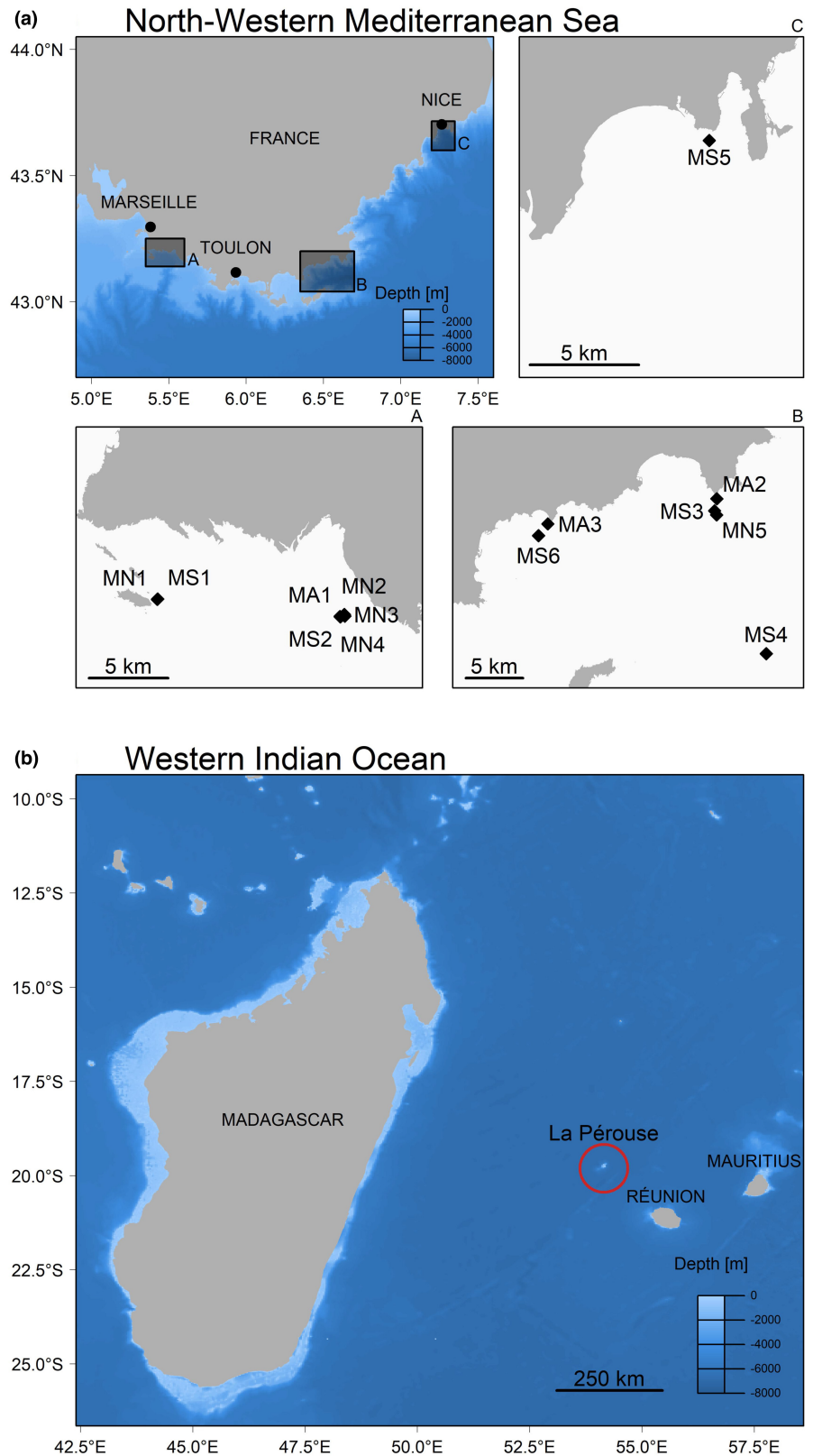
FIGURE 1 Area of eDNA sampling (a) in the coastal North-Western Mediterranean Sea and (b) at the seamount La P erouse in the Western Indian Ocean. More information about the sampling protocol can be found in supplementary material 1 (Tables S1 and S2; GEBCO Bathymetric Compilation Group 2021, 2021)
