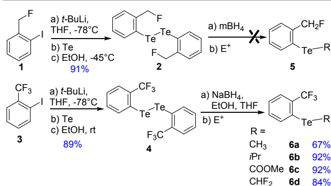
Scheme 1 Synthesis of a series of fluorinated alkyl aryl tellurides
