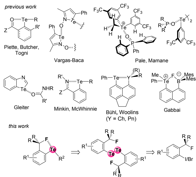
Fig. 2 The known noncovalent interactions involving tellurium atoms, and the first Te...F interaction described here.
