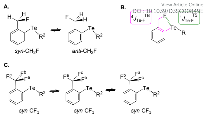
Fig. 3 (A) The more stable syn and anti conformations for the CH 2 F series. (B) Through bond (TB) and through space (TS) coupling for the syn conformation in the CH 2 F series. (C) Permanent syn conformation in the CF 3 series.
