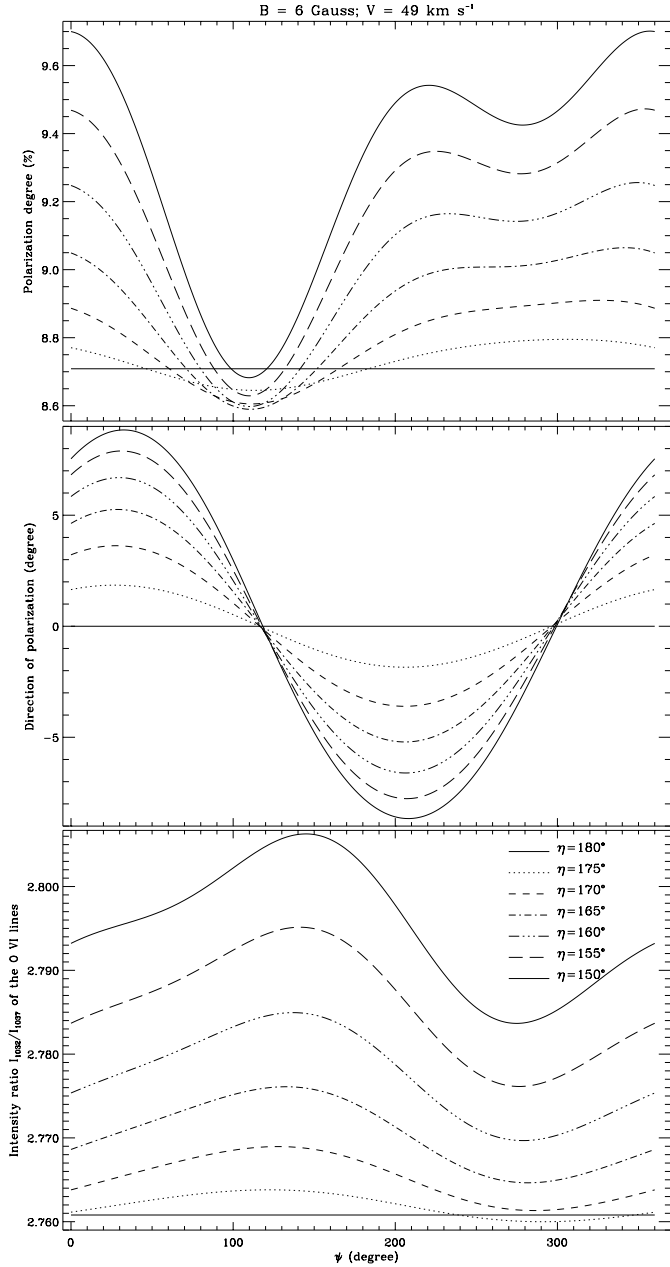
Fig. 8. The same as Fig. 5 but for a magnetic field of 6 Gauss combined with a velocity field vector of 49 \text{ km s}^{-1} .
