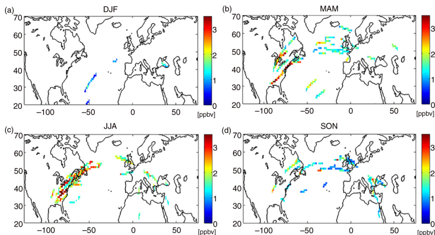
Fig. 8. Seasonally averaged NO y mixing ratios (ppbv) in the LSPs determined as described in Section 3. Values are averaged over 1° latitude × 1° longitude and for each season over the North mid-latitudes.
