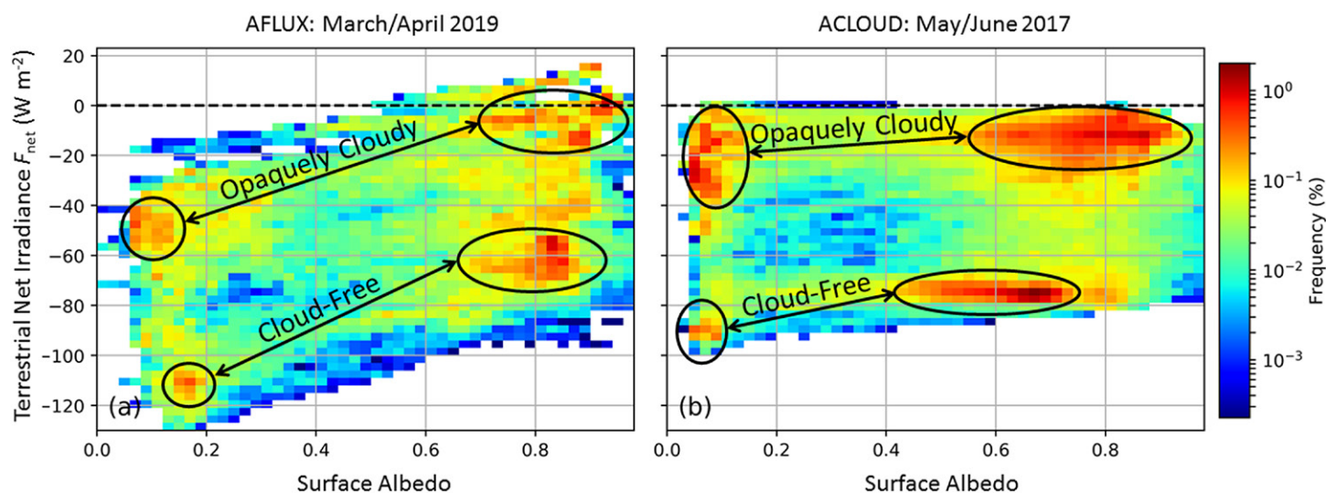
Fig. 8. Joint two-dimensional histogram of frequency distribution of terrestrial net irradiance (measured below clouds) as a function of all-sky surface albedo observed during (a) AFLUX and (b) ACLOUD. Two modes (cloud-free and opaquely cloudy) become obvious over both open ocean (low surface albedo) and sea ice (high surface albedo). The figure is taken from Stapf (2021).
