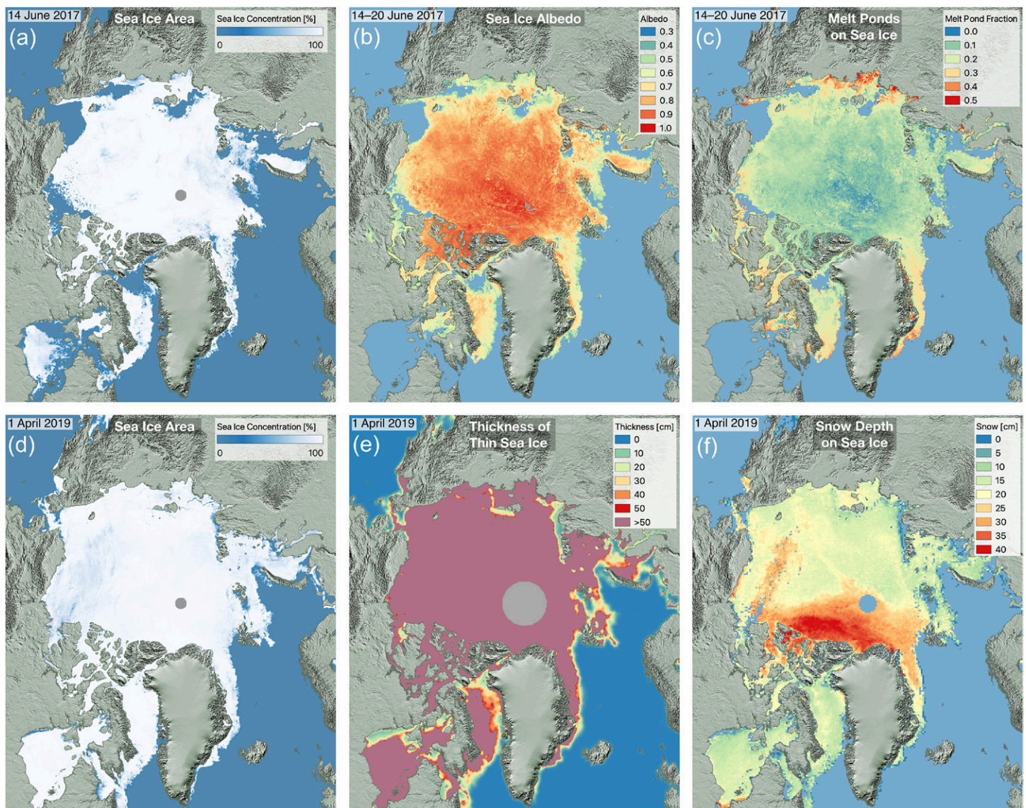
Fig. 4. Sea ice conditions from satellite observations during the (a)–(c) ACLOUD and (d)–(f) AFLUX campaigns. (a),(d) Sea ice concentration from the AMSR2 microwave radiometer. (b),(c) Sea ice albedo and fractional coverage of melt ponds on the sea ice from Sentinel-3 data (Pohl et al. 2020). (e) Thickness of thin sea ice from combined SMAP and SMOS L-band radiometer observations (Pařilea et al. 2019). (f) Snow depth on sea ice from AMSR2 observations (Rostosky et al. 2018, 2020). All data are available from https://seaice.uni-bremen.de .
