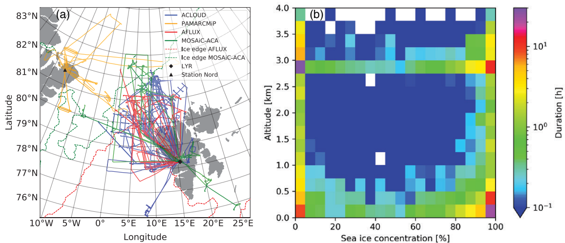
Fig. 3. Horizontal and vertical coverage of the aircraft observations conducted during ACLOUD (82 + 82 flight hours with Polar 5 and Polar 6), PAMARCMiP (40 flight hours, Polar 5), AFLUX (66 flight hours, Polar 5), and MOSAiC-ACA (44 flight hours, Polar 5); altogether 314 h of measurements (about 10% within clouds) were collected. (a) Horizontal projections of flight pattern during the airborne measurements; Lyr refers to Longyearbyen on Svalbard; (b) vertical distribution of number of flight hours spent in different altitudes over different sea ice conditions.
