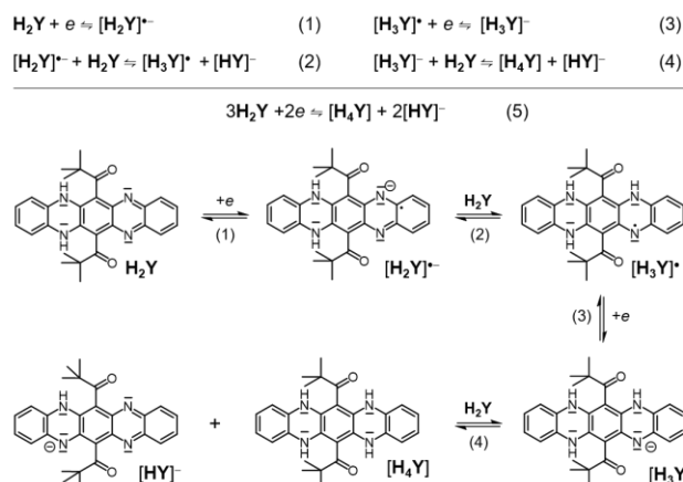
Fig. 14. Proposed mechanism following the reduction of \text{H}_2\text{Y} .
