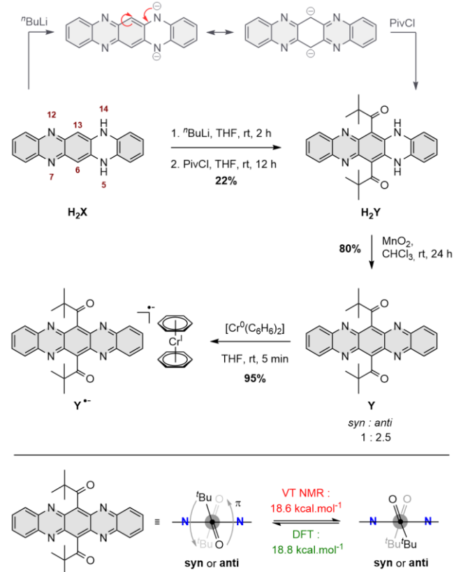
Fig. 2. Top: Synthesis of H2Y , Y and [\text{Y}]^{\cdot-} ; Bottom: Rotational barrier energy for the syn/anti isomers. The DFT barrier was obtained by a relaxed PCM(DMF)-M06/6-311G(d,p) scan.
