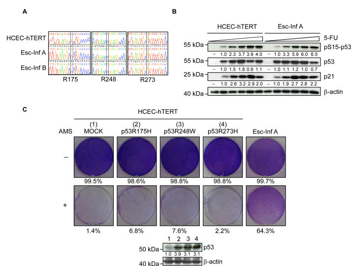
Figure 2. Escape from chronic-inflammation-induced senescence does not rely on p53 inactivation. (A) Confirmation of the wild-type status of the TP53 gene in HCEC-hTERT cells and their derivatives. TP53 exons within parental HCEC-hTERT cells and their Esc-Inf derivatives (of two independent experiments, Esc-Inf A and B) were fully sequenced. No mutation in TP53 was found, as shown by the sequences encompassing the exons encoding the residues R175, R248, and R273 that constitute the main mutation hot-spots reported in colitis-associated colon cancers. (B) The functionality of the p53 pathway in both parental HCEC-hTERT and its Esc-Inf derivatives was compared by submitting cells to an increasing dose of Fluorouracil (5-FU) over 24 h. The phosphorylation of the Ser10 of p53 (pS15-p53) and the levels of p53 and p21 CIP1 (p21) were assessed by Western blot. Protein levels were quantified relative to the \beta -actin and HCEC-hTERT cells. (C) The ectopic expression of p53 variants does not facilitate the escape of HCEC-hTERT cells from chronic-inflammation-induced senescence. Upper panels: cells were successively infected with mutant p53 retroviral-expressing vectors (as indicated on top), cultured in the presence of activated macrophage supernatants (+AMS) for ten days, and stained with crystal violet. Esc-Inf cells were used as an internal positive control. Percentages of stained surface are indicated. Lower panel: analysis of p53 by Western blot. Protein levels were quantified relative to the \beta -actin and HCEC-hTERT cells. Uncropped Western blots are provided in Supplementary File S2.
