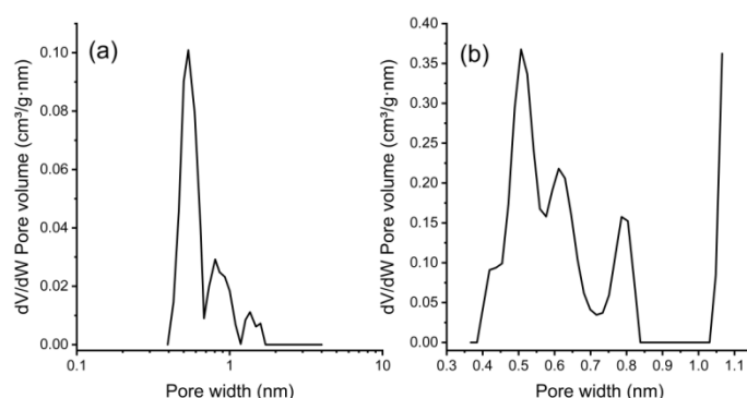
Figure 14. Pore size distributions of 2@1200 as obtained by DFT analysis of the N 2 sorption isotherms at -196\text{ }^{\circ}\text{C} (a) and CO 2 sorption isotherms at 0\text{ }^{\circ}\text{C} (b).
