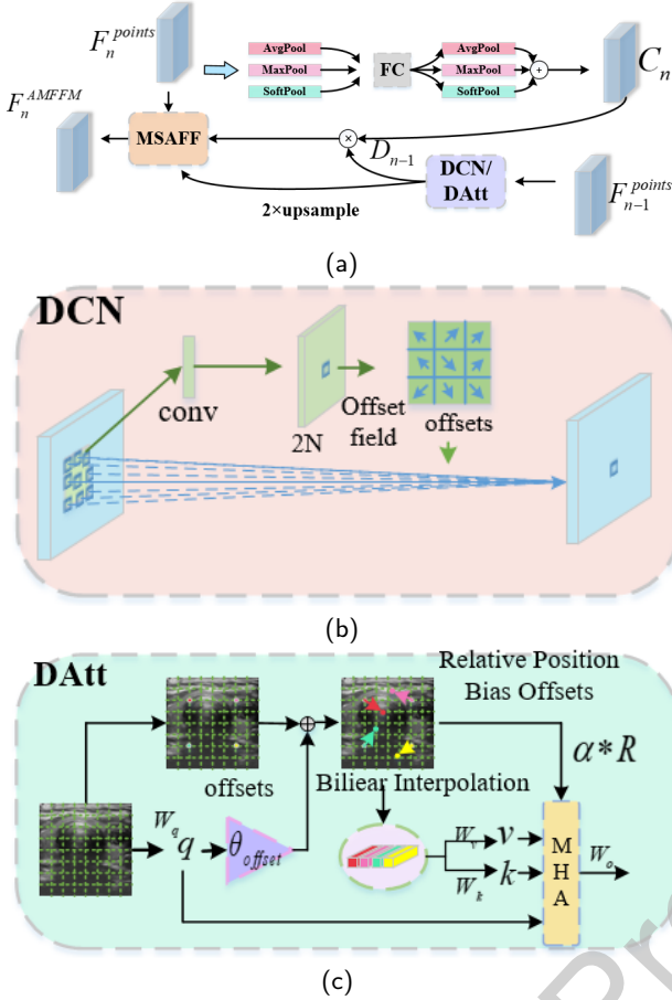
Figure 4: Adaptive Multi-scale Feature Fusion Module. (a) The overall structure of the Adapted Multi-scale Feature Fusion Module. (b) Details of Deformable Convolutions. (c) Details of Our Deformable Attention.
