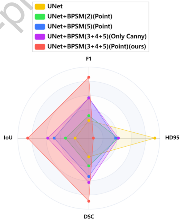
Figure 10: Radar chart of different placement of our Boundary Points Supervision Module.
