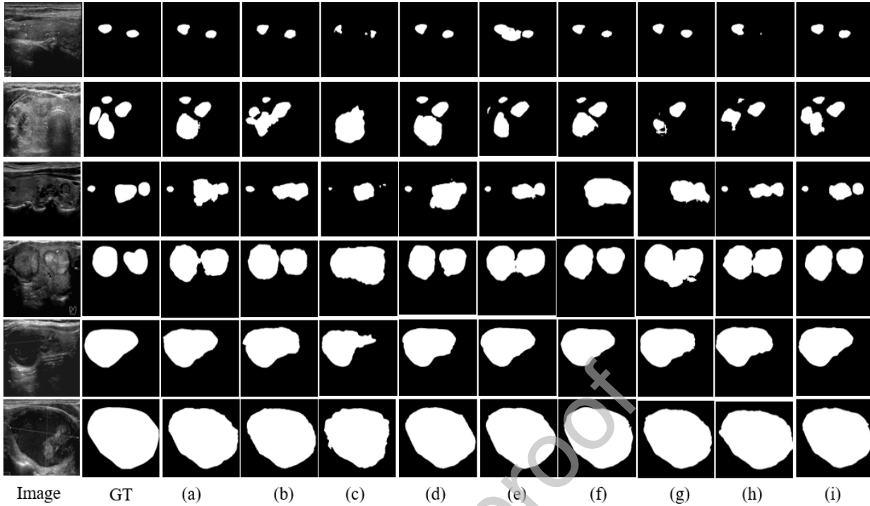
Figure 6: Segmentation results of different existing ways and our method on the TN3k dataset. (a) UNet. (b) FCN (c) Deeplabv3-Resnet50. (d) AttnUNet. (e) SmaAt-UNet. (f) UT-Net. (g) UNet Transformer. (h) TransUNet (i). BPAT-UNet.
