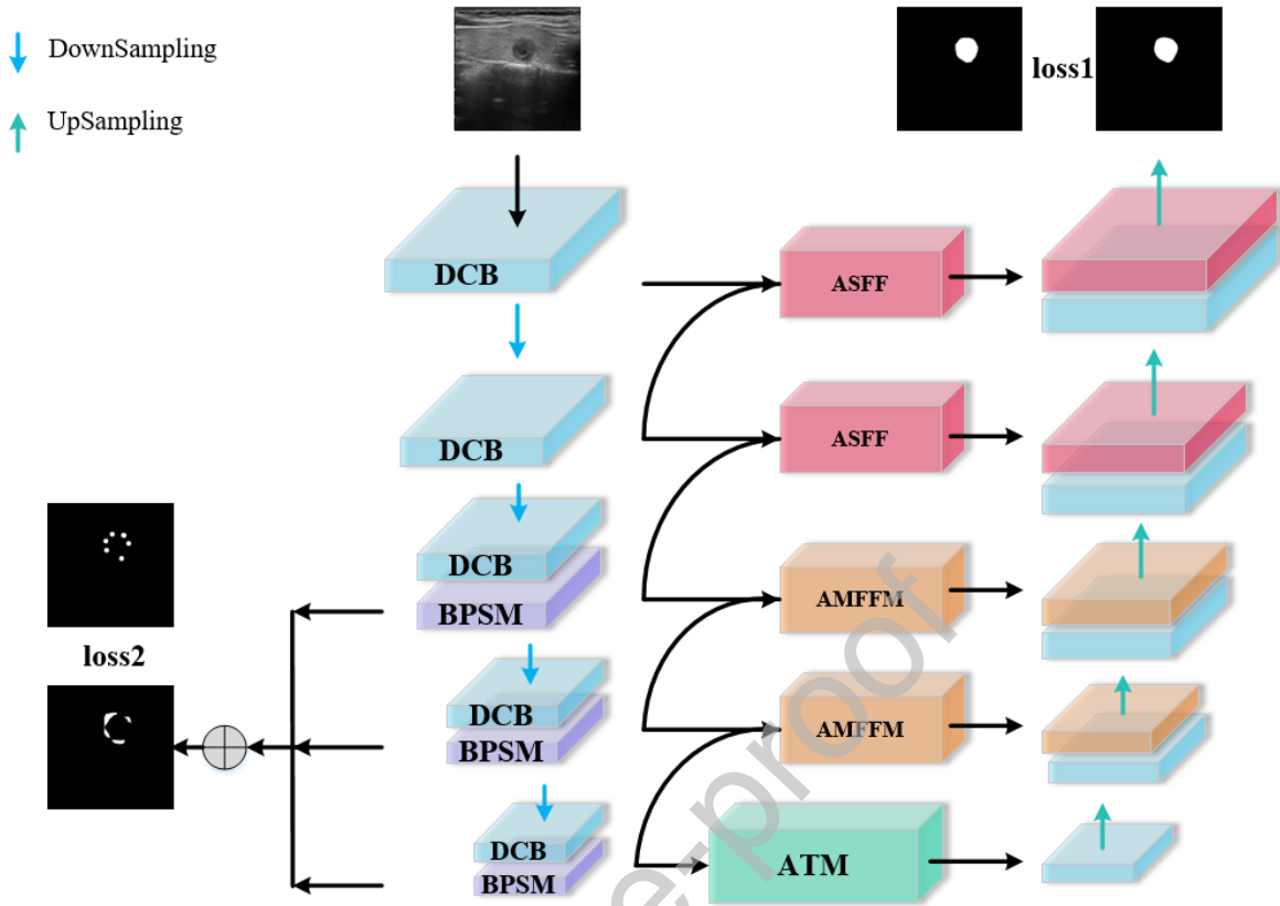
Figure 2: Overall architecture of our proposed BPAT-UNet.
