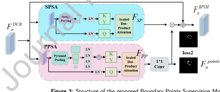
Figure 3: Structure of the proposed Boundary Points Supervision Module in detail.
