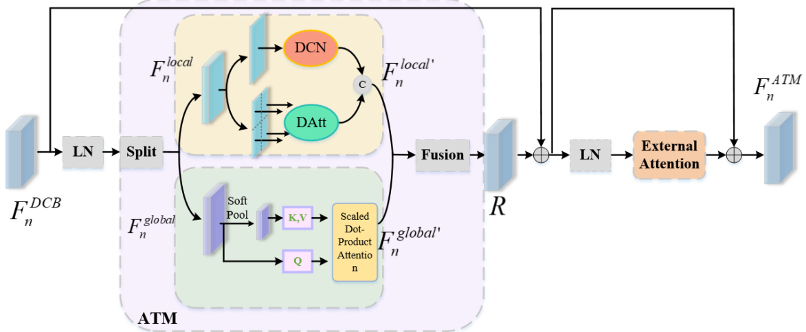
Figure 5: Details of Assembled Transformer Module.
