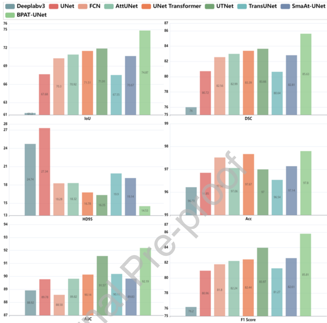
Figure 9: Visualization of evaluation metrics of the compared methods and the proposed BPAT-UNet on the private thyroid ultrasound dataset.
