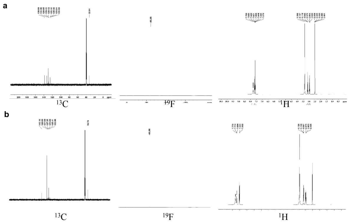
Figure S1. NMR measurement of a) ( m -CF 3 PEA) 2 PbI 4 and b) ( p -CF 3 PEA) 2 PbI 4 films.
