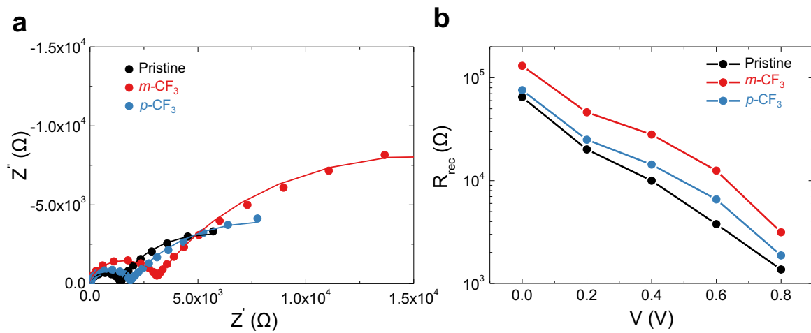
Figure S21. (a) Nyquist plots from EIS measurements with an applied voltage of 0.4 V. (b) Voltage dependent surface recombination resistance ( R_{s, \text{Rec}} ) of the devices using pristine perovskite films, m\text{-CF}_3 PEAI treated- and p\text{-CF}_3 PEAI treated perovskite films.
