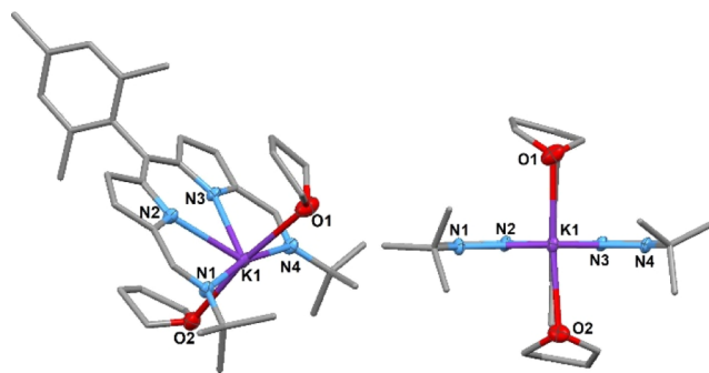
Figure 2. Solid-state structure of K(L Mes )·(THF) 2 viewed from the top (left) and side (right). For clarity, all hydrogen atoms and one molecule are omitted (displacement ellipsoids are drawn at 50% probability). Selected bonds (Å) and angles (deg): K1–N1, 2.897(3); K1–N2, 2.732(4); K1–N3, 2.715(3); K1–N4, 2.916(3); K1–O1, 2.761(3); K1–O2, 2.799(3); N1–K1–N2, 61.65(9); N2–K1–N3, 66.40(9); N3–K1–N4, 62.28(9); N4–K1–N1, 169.56(9); O1–K1–O2, 171.36(9); C20–C10–C9, 128.2(4); C9–C10–C11, 116.5(4); and C11–C10–C20, 115.3(4).
