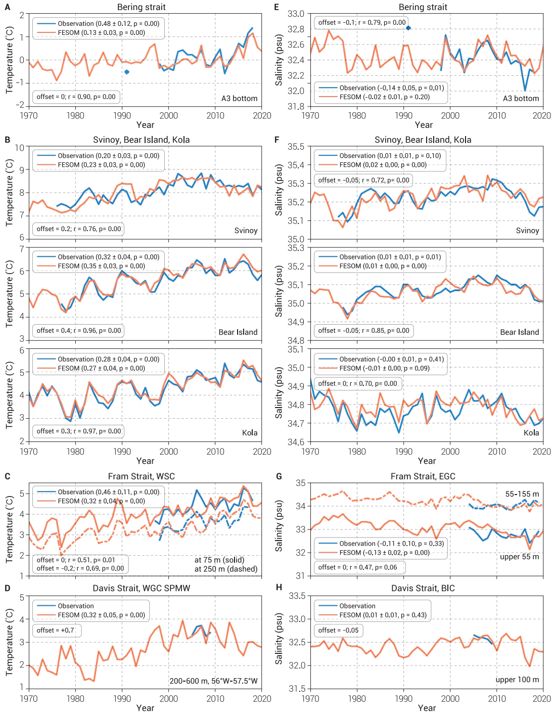
Figure 2: Annual-mean (left) potential temperature and (right) salinity. (A), (E) Temperature and salinity at the bottom of the Bering Strait. (B), (F) Temperature and salinity at 50–200 m in the Svinoy, Bear Island and Kola sections (from top to bottom). (C) Temperature at 75 m (solid) and 250 m (dashed) depths in the core of the West Spitsbergen Current in the Fram Strait. (G) Salinity in the upper 55 m (solid) and 55–155 m (dashed) depths in the East Greenland Current in the Fram Strait. (D) Temperature of the Subpolar Mode Water in the West Greenland Current in the Davis Strait. (H) Salinity in the upper 100 m in the Baffin Island Current in the Davis Strait. Observations are in blue, and FESOM simulated results are in red (see Section 2 for data references and descriptions). The offsets added to the model results for plotting are indicated in the panels. The correlation coefficients between the observations and model results are indicated with r . In legends, the linear trends over the periods of the model (1970 to 2020) and the observations (variable, see the length of blue lines) are cited.
