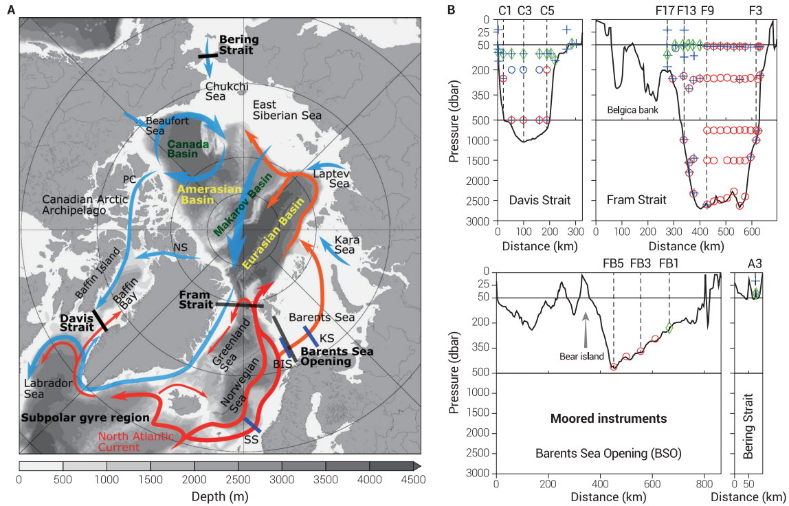
Figure 1: (A) Schematic of pan-Arctic Ocean circulations. Blue arrows denote upper ocean circulation, and red arrows denote Atlantic Water circulation. The background gray color denotes bottom bathymetry. The four Arctic gateways reviewed in this paper (Bering, Fram and Davis straits, and the Barents Sea Opening) are indicated with black lines. SS: Svinoy Section; BIS: Bear Island Section; KS: Kola Section; NS: Nares Strait; PC: Parry Channel. (B) Location of mooring instruments in the four Arctic gateways (indicated by black lines in (A)). Red circles depict single-point current meters that measure velocity and temperature. Blue circles depict current meters with both temperature and salinity sensors. Blue crosses depict SeaBird MicroCAT devices that measure temperature and salinity. Green diamonds depict ADCPs, which measure velocity. (B) is modified from [16] (©American Meteorological Society; used with permission) with new instruments added.
