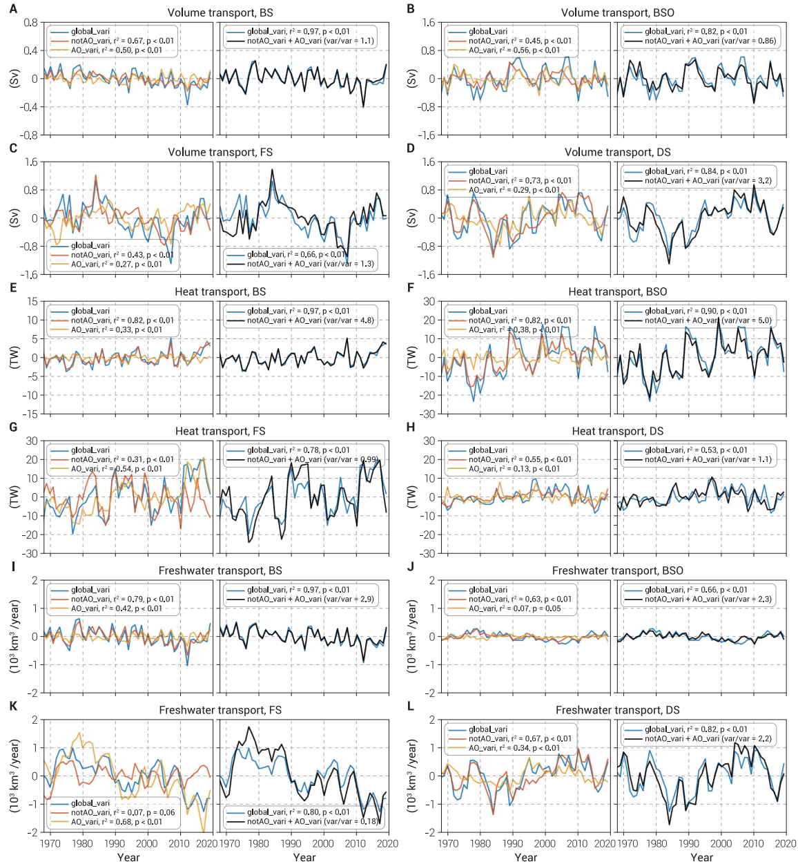
Figure 5: Anomalies of annual-mean ocean volume transport in the FESOM simulations: in the (A) Bering Strait (BS), Barents Sea Opening (BSO), (C) Fram Strait (FS) and (D) Davis Strait (DS). (E)–(H) The same as (A)–(D), but for heat transport (relative to 0°C). (I)–(L) The same as (A)–(D), but for freshwater transport (relative to 34.8). In each panel, the left plot shows the results of individual experiments: global_vari (historical simulation), notAO_vari in which atmospheric forcing has interannual variability outside the Arctic, but not inside the Arctic, and AO_vari in which forcing has interannual variability inside the Arctic, but not outside the Arctic. The fractions of explained variance are shown in the legends ( r^2 ). In each panel, the right plot depicts the historical simulation and the sum of the two sensitivity experiments. The fractions of explained variance ( r^2 of the two lines) and the ratio of the individual variances between notAO_vari and AO_vari are shown in the legends.
