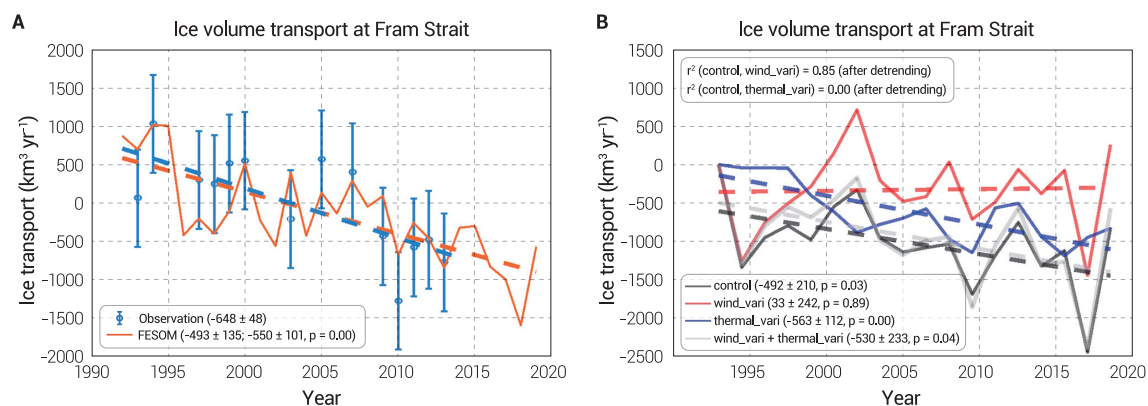
Figure 4: (A) Anomaly of annual-mean sea ice volume transport in the Fram Strait: Observations in blue and FESOM historical simulation in red. The dashed lines depict the linear fit, with the trends shown in the legend. The trends in the model are calculated for the period of available observations and for the whole illustrated period as well. (B) Winter-centered annual-mean sea ice volume transport in the Fram Strait in FESOM simulations: (black) control (historical) simulation; (red) sensitivity simulation in which winds have interannual variability, but Arctic thermal forcing is climatology; (blue) sensitivity simulation in which thermal forcing has interannual variability, but Arctic winds are climatology; (gray) sum of the red and blue lines. The anomalies relative to the first year are shown. The dashed lines depict the linear fit, and the trends are shown in the legend. The fractions of the variance in the control simulation that can be explained by the two sensitivity simulations are shown at the top of the plot ( r^2 ). In this figure, Arctic sea ice export is defined to be positive, so a downward trend indicates a reduction in sea ice export. The figure is modified from Wang et al. [182]. The observation data in (A) were described by Spreen et al. [26].
