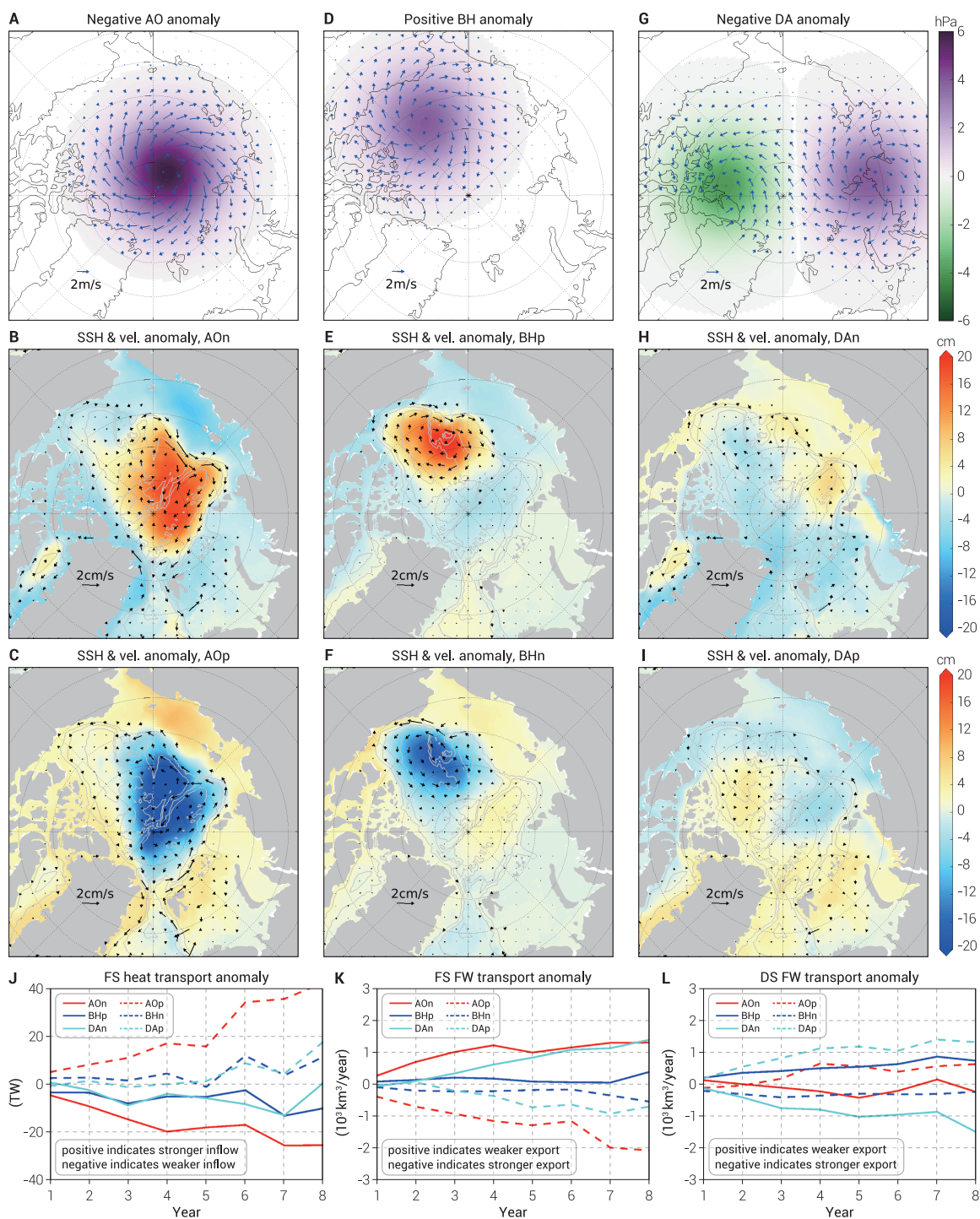
Figure 6: Winds representing the (A) negative phase of the Arctic Oscillation, (D) positive Beaufort High anomaly, and (G) negative phase of the Arctic Dipole Anomaly that are used in the wind-perturbation experiments. The associated sea level pressure anomalies are also depicted. Sea surface height and velocity differences between the wind-perturbation experiments and the control run: perturbed with the (B) negative Arctic Oscillation forcing (AOn), (C) positive Arctic Oscillation forcing (AOp), (E) positive Beaufort High anomaly (BHp), (F) negative Beaufort High anomaly (BHn), (H) negative Dipole Anomaly forcing (DAn), and (I) positive Dipole Anomaly forcing (DAp). (J) Anomalies of heat transport in the Fram Strait relative to the control run. (K) Anomalies of freshwater transport in the Fram Strait relative to the control run. (L) The same as (K), but for the Davis Strait. Ocean heat and freshwater transports are calculated relative to 0^\circ\text{C} and 34.8 , respectively.
