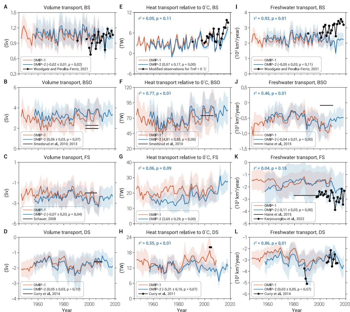
Figure 3: Simulated annual-mean ocean volume transport (left), heat transport (middle, relative to 0°C) and freshwater transport (right, relative to 34.8) in OMIP1 (red) and OMIP2 (blue) models. From top to bottom: Bering Strait (BS), Barents Sea Opening (BSO), Fram Strait (FS), and Davis Strait (DS). The multi-model-mean results are given together with model spreads as background shading. The linear trends of the OMIP2 results from 1970–2018 are shown in the legends. r^2 values in the middle and right columns indicate the coefficient of determination between ocean volume transport and the corresponding heat/freshwater transport in OMIP2. Available observations are also shown. Note that the observed Bering Strait heat transport was modified from the original data by changing the reference temperature to 0°C, and the original Bering Strait heat transports relative to -1.9^\circ\text{C} are approximately 8 TW higher than the numbers presented here. Positive values indicate inflows to the Arctic Ocean. The model data used in this figure are described by Shu et al. [124].
