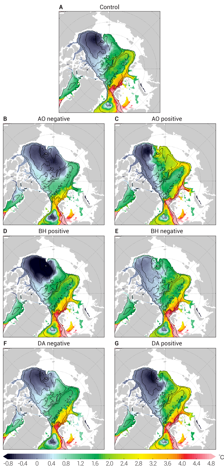
Figure 7: Temperature at 300 m depth in the last model (8th) year in (A) the control simulation and in experiments perturbed with winds of the (B) negative Arctic Oscillation, (C) positive Arctic Oscillation, (D) positive Beaufort High anomaly, (E) negative Beaufort High anomaly, (F) negative Dipole Anomaly, and (G) positive Dipole Anomaly.
