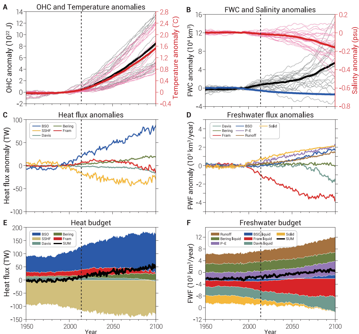
Figure 8: CMIP6 historical and SSP585 results (periods separated by the vertical dashed lines). Anomalies of the Arctic Ocean (A) heat content [black] and temperature [red], (B) liquid [black] and solid [blue] freshwater contents and salinity [red], (C) heat budget terms, and (D) freshwater budget terms. The anomalies are relative to 1980–2000 means. (E) Arctic Ocean heat budget. (F) Arctic Ocean freshwater budget. Ocean heat and freshwater transports are calculated relative to 0^{\circ} C and 34.8, respectively. In (A) and (B), the thin lines represent the results of individual models to illustrate the large model spreads. The model data used in this figure are described by Shu et al. [75] and Wang et al. [126]. OHC: ocean heat content; FWC: freshwater content; BSO: Barents Sea Opening; SSHF: sea surface heat flux; P-E: precipitation minus evaporation.
