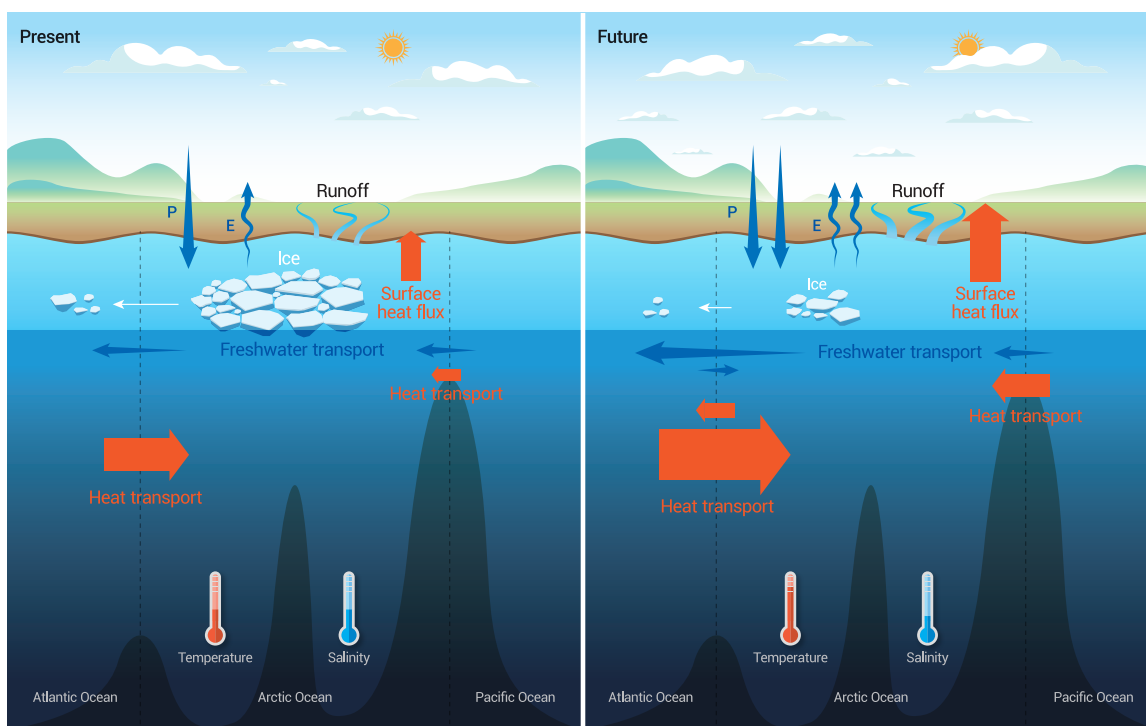
Figure 9: Schematic showing changes in Arctic Ocean heat (red arrows) and freshwater (blue arrows) budgets in a warming climate. The poleward ocean heat convergence and the hydrological cycle are strengthened with climate warming. P: precipitation; E: evaporation.
