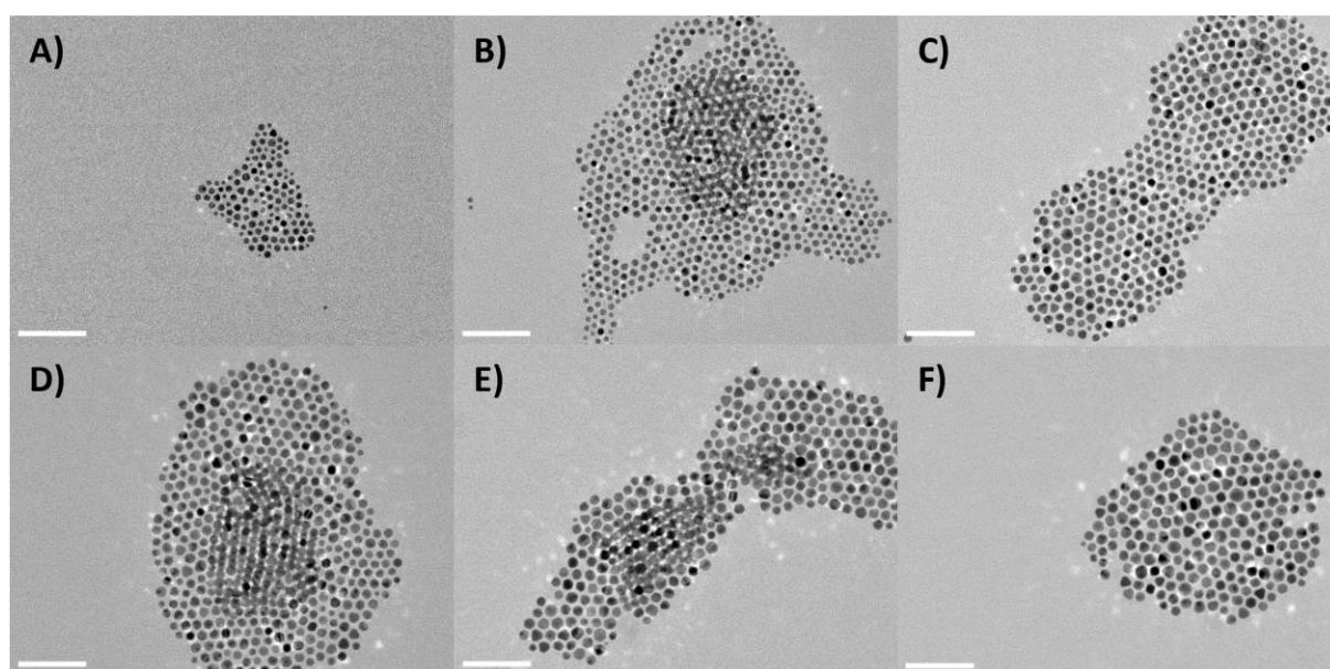
Figure 7. TEM images of the AuNPs seeds (A), obtained for a \text{Me}_2\text{S}\cdot\text{AuCl}:\text{NHC}\text{-BH}_3 ratio of 1:28 and after each subsequent addition of \text{Me}_2\text{S}\cdot\text{AuCl} (B to F). Scale bars are 50 nm.
