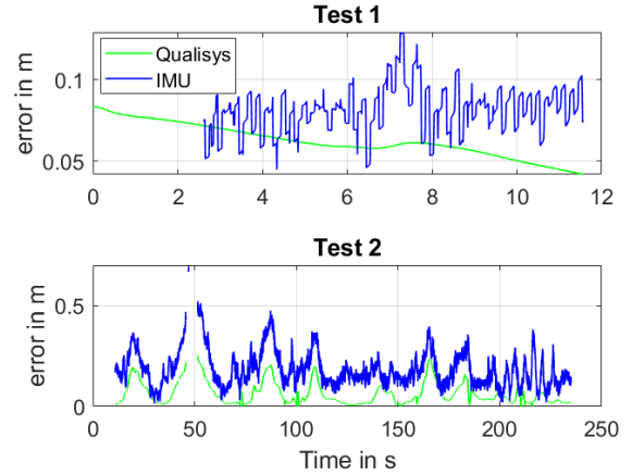
Figure 10: Comparison of the average error of position estimated by the Qualisys and the IMU. Average error with IMUs: E_d = 0.08\text{m} for Test1 and E_d = 0.18\text{m} for Test2. Average error with Qualisys: E_d = 0.062\text{m} for Test1 and E_d = 0.065\text{m} for Test2.
