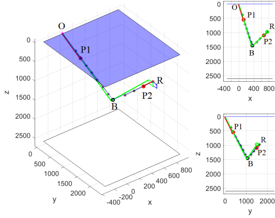
(a) With sliding mass
