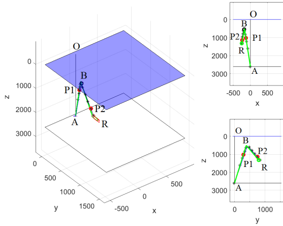
(b) With sliding buoy
