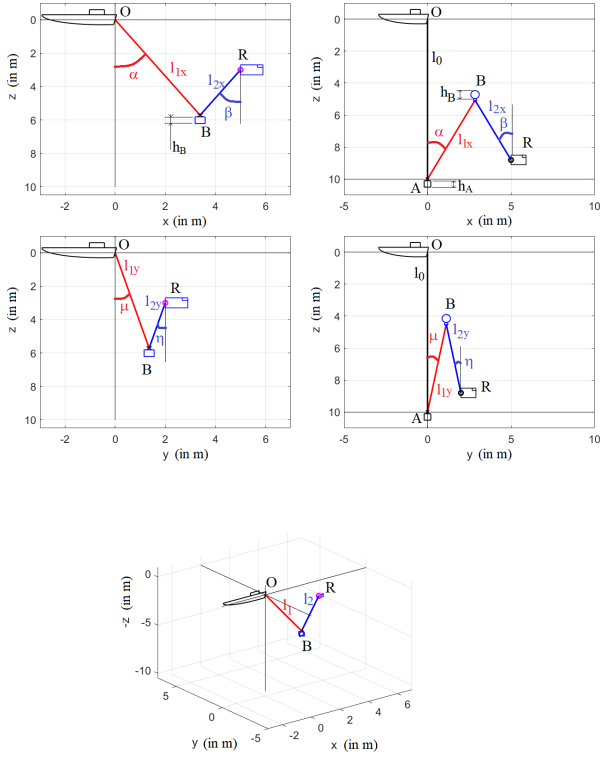
Figure 1: Parameters for a sliding ballast or buoy for (x, y, z)=(5, 2, 3) , L = 10 and l_0 = 0 in the ballast case, and (x, y, z)=(5, 2, 8.8) , L = 10 and l_0 = L in the buoy case. R : ROV. B : sliding ballast or buoy. The black, red and blue lines correspond to l_0 , l_1 , l_2 . l_{1x} , l_{1y} , l_{2x} , l_{2y} are the projections of l_1 and l_2 on the plane (O, \vec{x}, \vec{z}) and (O, \vec{y}, \vec{z}) .
