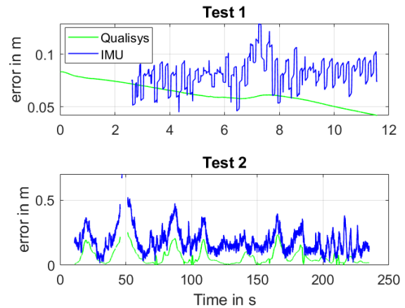
Figure 10: Comparison of the average error of position estimated by the Qualisys and the IMU. Average error with IMUs: E_d = 0.08\text{m} for Test1 and E_d = 0.18\text{m} for Test2. Average error with Qualisys: E_d = 0.062\text{m} for Test1 and E_d = 0.065\text{m} for Test2.
