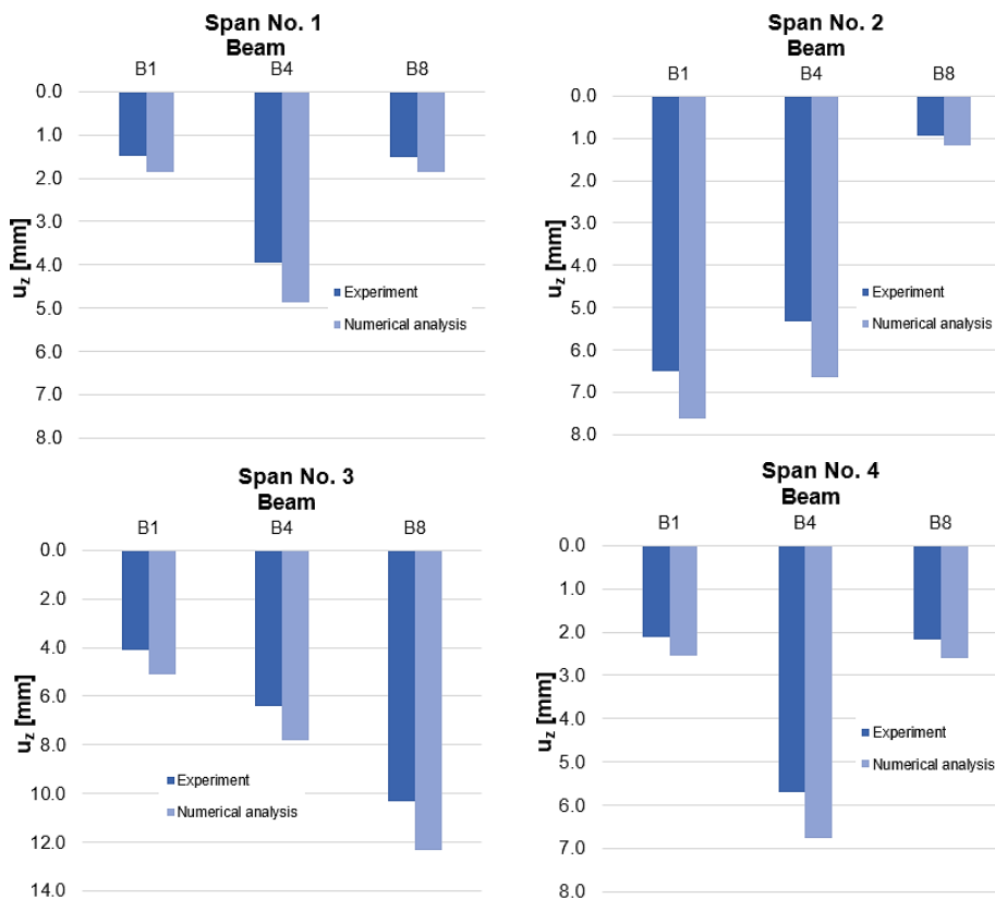
Fig. 11: Comparison of experiment and numerical analysis.
