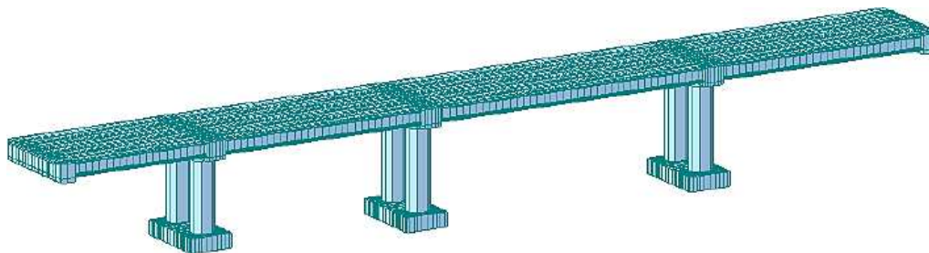
Fig. 6: FEM model of the bridge.
