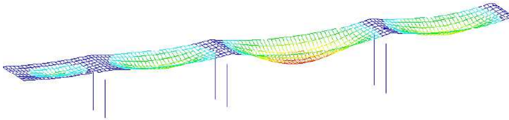
Fig. 7: Deflections due to the Test load in span No. 3.
