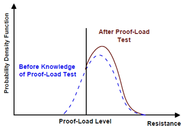
Fig. 2: Resistance after proof load test (Nowak and Tharmabala, 1998).
