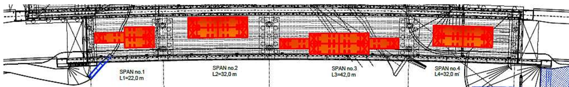
Span no.1 – 3 vehicles, Span no. 2 – 4 vehicles, Span no.3 – 6 vehicles, Span no.4 – 4 vehicles.
