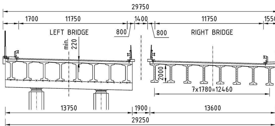
Fig. 5: Cross-section of the bridge [mm].
