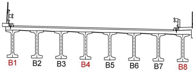
Fig. 8: Cross-section: Position of deflection measurements.
