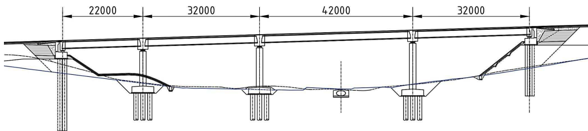
Fig. 4: Longitudinal section of the bridge [mm].
