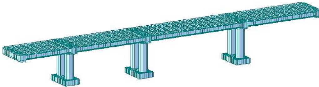
Fig. 6: FEM model of the bridge.
