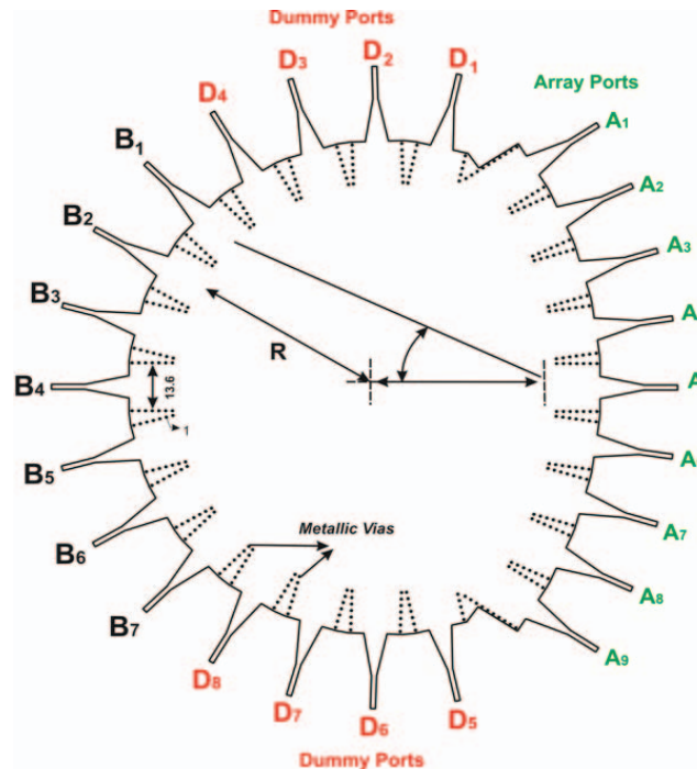
Fig. 1. Geometry of the realized SIW Rotman lens
