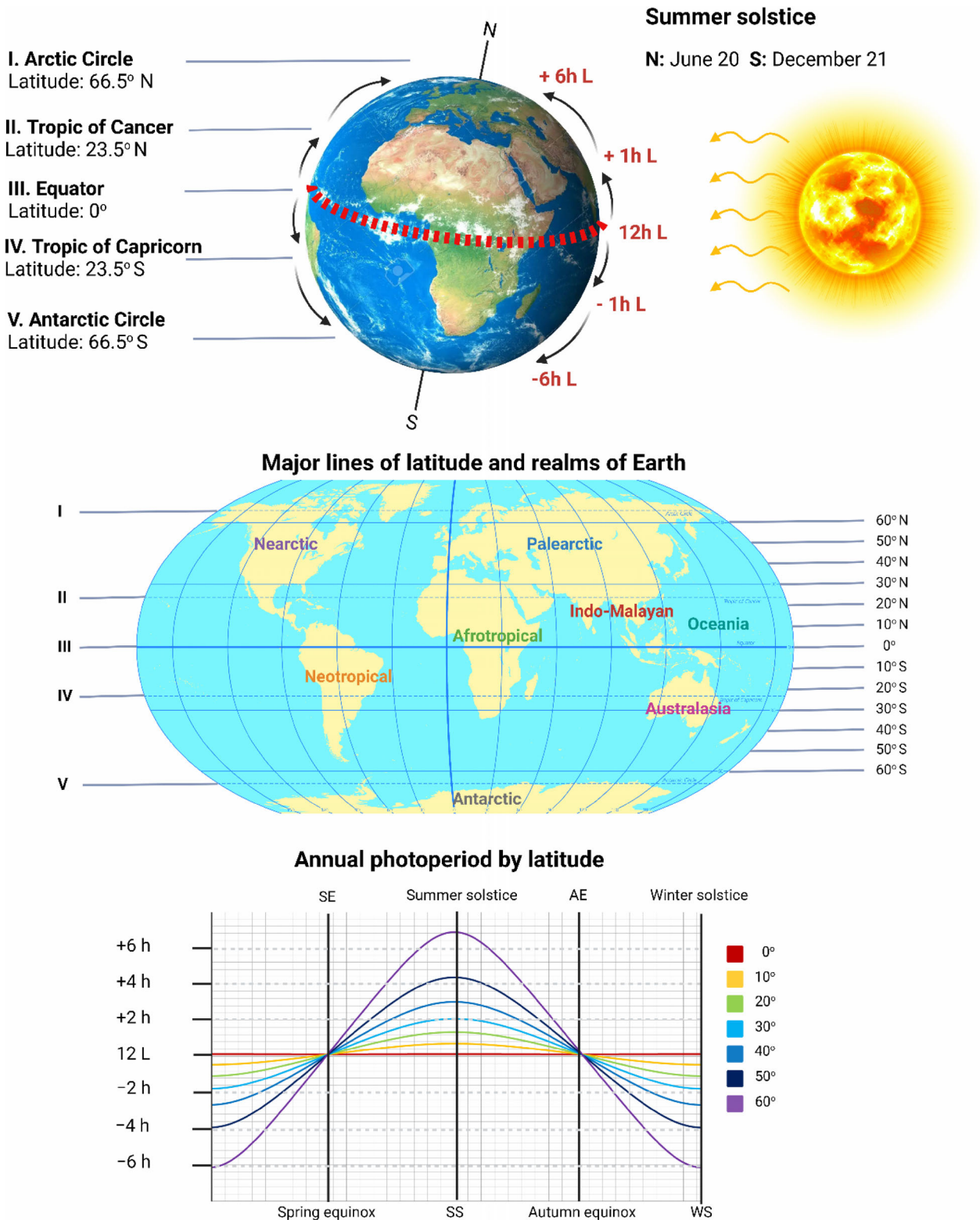
Fig. 2. Diagrammatic representation of the major lines of latitude of Earth and the relative photoperiod at each latitude between the four key dates for changing photoperiods. In the top panel, the orientation of the Earth at the summer solstice is indicated with the difference in day length between the equator (broken line) and the two major tropics and the polar circles. In the centre panel, these lines are indicated on a map, along with the intermediate lines of latitude. In the bottom panel, the annual variation in photoperiod is plotted for each 10° increment in latitude across the year. (Created with BioRender.com ).
