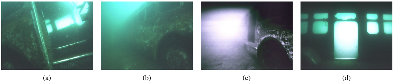
Fig. 2: Bus dataset [3]
