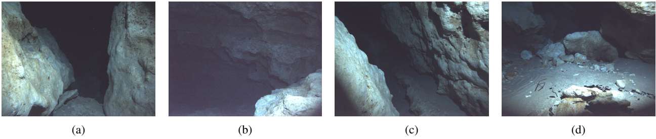
Fig. 3: Cave dataset [3]
