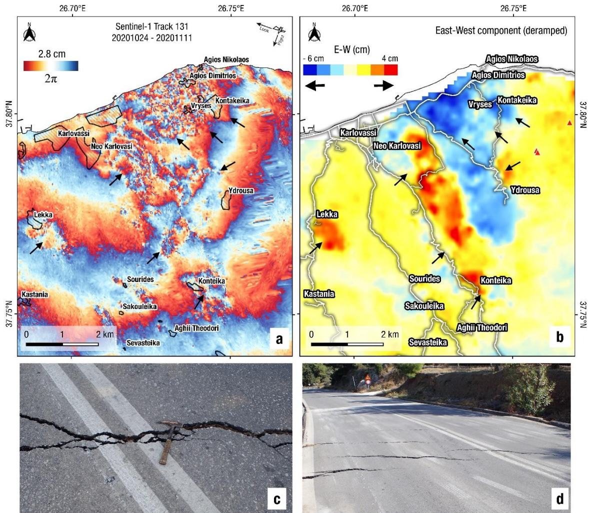
511 Fig. 11. Maps showing co-seismic landslide activity around Karlovasi, evident in Sentinel-1 512 differential interferograms. De-correlated areas and fringe patterns mark the location of 513 DSGDs (black arrows) in descending (a) interferogram. Decomposed unwrapped 514 interferograms (East – West component) show the extent of triggered landslides (b). The 515 E-W displacement raster image was deramped around the landslide area in order to 516 diminish the co-seismic displacement effect and to enhance movement along the eastern 517 and western slopes. c & d) Field photos of ground cracks along the boundaries of activated 518 landslides (see Table S4 for coordinates).
