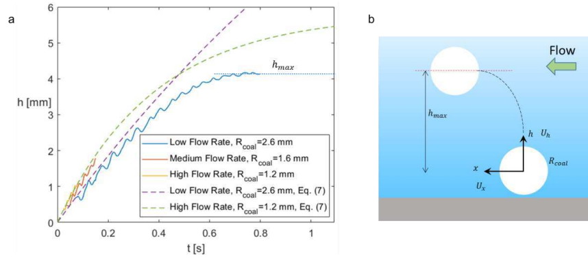
FIG. 13: (a) The temporal variation of CG height of the bubble in shear flow at different liquid flow rate conditions post jumping of the bubbles from the substrate. (b) The schematic of the rising motion of the bubble post jumping.
