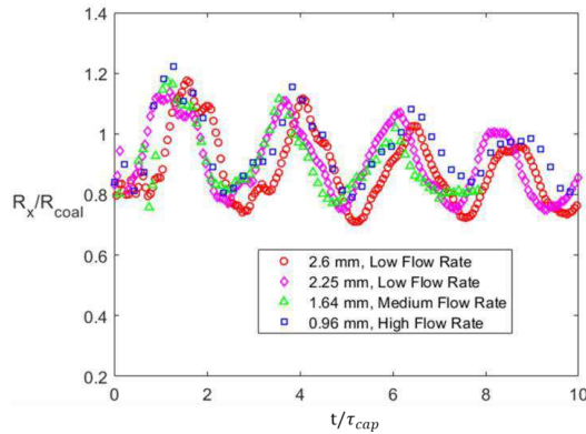
FIG. 11: Variation of non-dimensional bubble radius ( R_x/R_{coal} ) during oscillation versus time normalized with respect to capillary time scale for different bubble size R_{coal} at lift-off.
