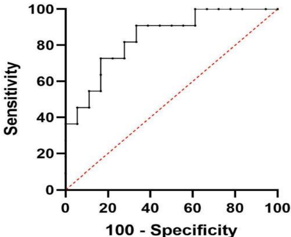
Figure 3 Receiver operating characteristic curve for admission troponin between severe and non-severe patients.
