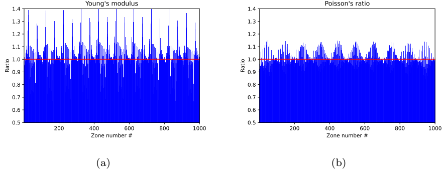
Figure 8: Ratio comparison for the 3D example 1
