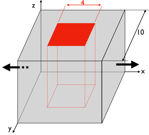
Figure 7: Configuration of 3D example 1. The core of the cube (red zones) which contains 160 zones: E = 2 MPa and \nu = 0.3 ; The rest part (grey zones): E = 1 MPa and \nu = 0.3 ; loading: \sigma_{xx} = (0.1y + 0.5) MPa.
