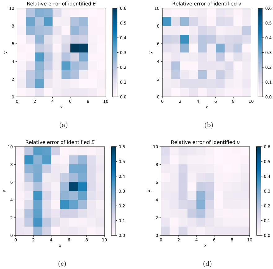
Figure 6: Comparison of e_r between two variants for RP3. (a),(b): Variant 1; (c),(d): Variant 2.
