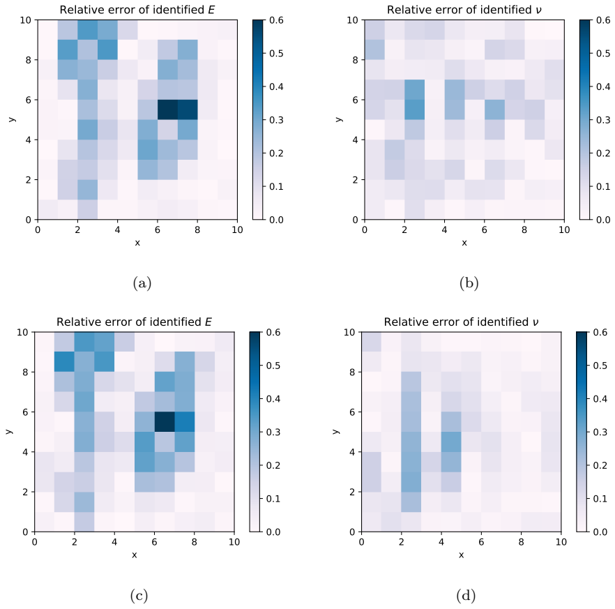
Figure 5: Comparison of e_r between two variants for RP2. (a),(b): Variant 1; (c),(d): Variant 2.
