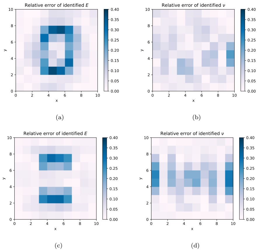
Figure 4: Comparison of e_r between two variants for RP1. (a),(b): Variant 1; (c),(d): Variant 2.
