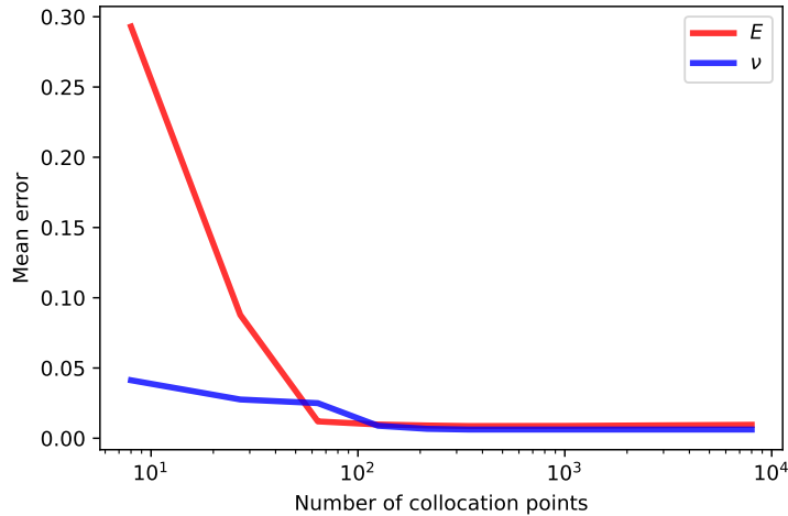
Figure 9: Mean error ( \frac{\sum e_r}{N_s} ) of identified parameters with different number of collocation points
