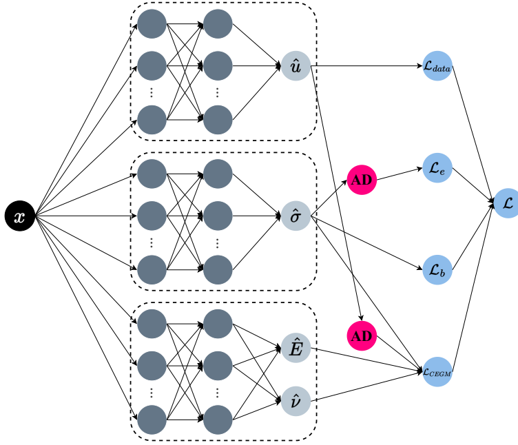
Figure 1: Forward propagation of identification using PINNs
