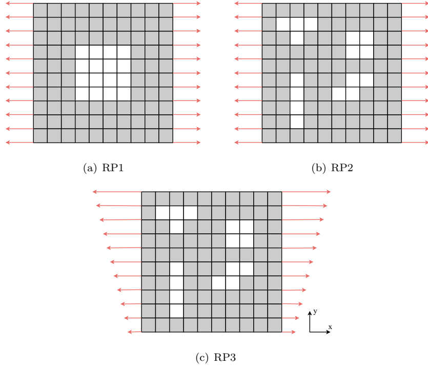
Figure 2: Maps of material heterogeneities and their loading. (a) White zones: E = 2 MPa and \nu = 0.3 ; grey zones: E = 1 MPa and \nu = 0.3 ; loading: \sigma_{xx} = 1 MPa. (b) White zones: E = 2 MPa and \nu = 0.3 ; grey zones: E = 1 MPa and \nu = 0.3 ; loading: \sigma_{xx} = 1 MPa. (c) White zones: E = 2 MPa and \nu = 0.3 ; grey zones: E = 1 MPa and \nu = 0.3 ; loading: \sigma_{xx} = (0.1y + 0.5) MPa.
