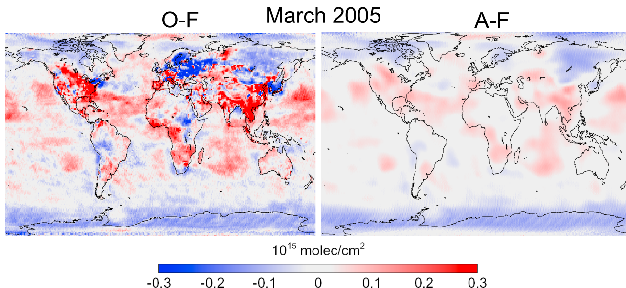
Figure 2. (left) Monthly mean observation-forecast (O – F) and (right) analysis-forecast (A – F) differences in NO 2 slant columns for March 2005 (1° × 1°). For each OMI pixel, the measured slant column (observation) and the model-predicted slant column (forecast) were divided by the same geometrical air mass factor.
