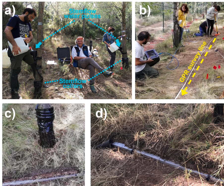
Fig. 2. (a): Stemflow water pulses poured on Trees 1 and 2. (b): GPR survey carried out on Survey line 2. (c): Stemflow collar. (d): Channel for collecting overland flow.
