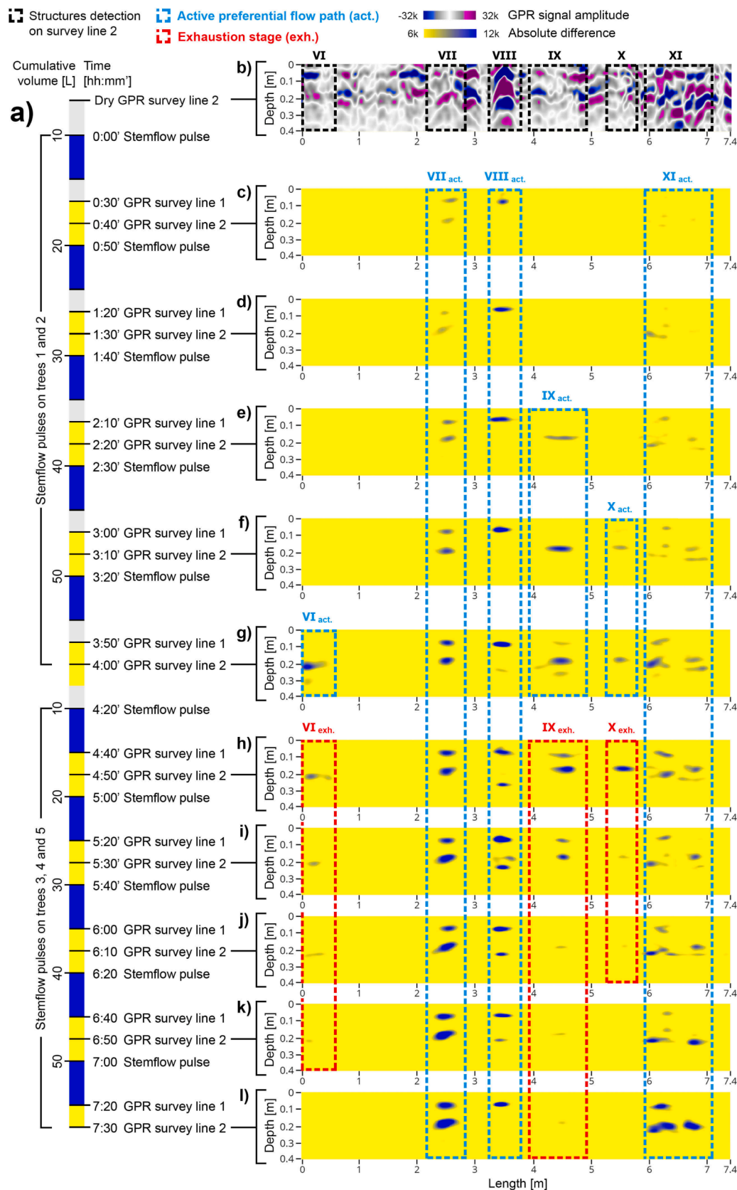
Fig. 5. (a): Timeline of the repeated GPR surveys and stemflow pulses for the GPR Survey line 2. (b): Radargram collected before the execution of the artificial stemflow experiment. (c-g): Differenced radargrams obtained during the first stage of the artificial stemflow experiment, when water was poured on Trees 1 and 2. (h-l): Differenced radargrams obtained during the second stage of the artificial stemflow experiment, when water was poured on Trees 3, 4 and 5. The positions of the coarse roots that triggered preferential flow paths are indicated with Roman numerals from VI to XI and black rectangles. The positions of the detected active preferential flow paths are indicated with Roman numerals followed by the subscript act. (active) and blue rectangles. The exhaustion stages are indicated with Roman numerals followed by the subscript exh. (exhaustion) and red rectangles. (For interpretation of the references to colour in this figure legend, the reader is referred to the web version of this article.)
