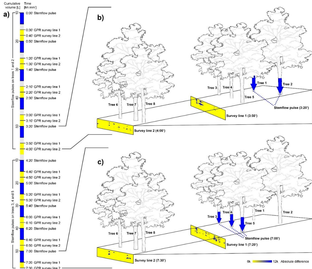
Figure 3. (a): Timeline of the repeated GPR surveys and stemflow pulses. (b): Differenced radargrams obtained at the end of the first stage of the artificial stemflow experiment, when water was poured on Trees 1 and 2 (blue arrows) at time 3:50' for Survey line 1 and 4:00' for Survey line 2. (c): Differenced radargrams obtained at the end of the second stage of the artificial stemflow experiment, when water was poured on Trees 3, 4, and 5 (blue arrows) at time 7:20' for Survey line 1 and 7:30' for Survey line 2.
