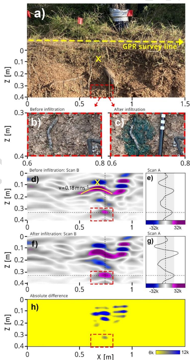
Figure 6. Dye-staining experiment. (a): Roadcutbank with the selected Aleppo pine tree located at around 0.7 m from the border. The dashed yellow arrow demarcates the 1.5-m-long survey line positioned at a distance of 0.3 m from the roadcutbank. A root that funneled the stemflow was photographed (b) before and (c) after the appearance of the brilliant blue dye (E133) solution. Radargrams (B-scans) were collected on a 1.5-m-long survey line (d) before and (f) after the execution of the artificial stemflow experiment. Reflection traces (A-scans) were collected (e) before and (g) after the execution of the artificial stemflow experiment in correspondence of the root that funneled the dye tracer. (h): Differenced radargram. The red rectangles demarcate the position of the root that funneled the stemflow. The yellow cross demarcates the position of a coarse root and of the corresponding adapted hyperbola.
