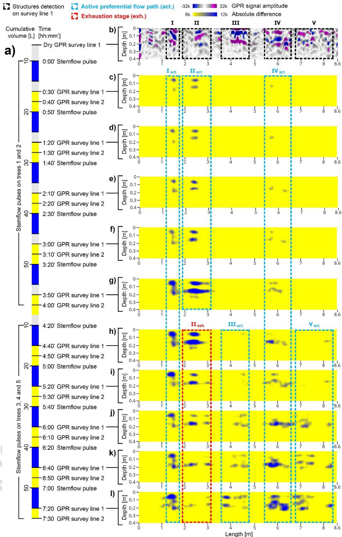
Figure 4. (a): Timeline of the repeated GPR surveys and stemflow pulses for the GPR Survey line 1. (b): Radargram collected before the execution of the artificial stemflow experiment. (c-g): Differenced radargrams obtained during the first stage of the artificial stemflow experiment, when water was poured on Trees 1 and 2. (h-l): Differenced radargrams obtained during the second stage of the artificial stemflow experiment, when water was poured on Trees 3, 4 and 5. The positions of the coarse roots that triggered preferential flow paths are indicated with Roman numerals from I to V and black rectangles. The positions of the detected active preferential flow paths are indicated with Roman numerals followed by the subscript act. (active) and blue rectangles. The exhaustion stages are indicated with Roman numerals followed by the subscript exh. (exhaustion) and red rectangles.
