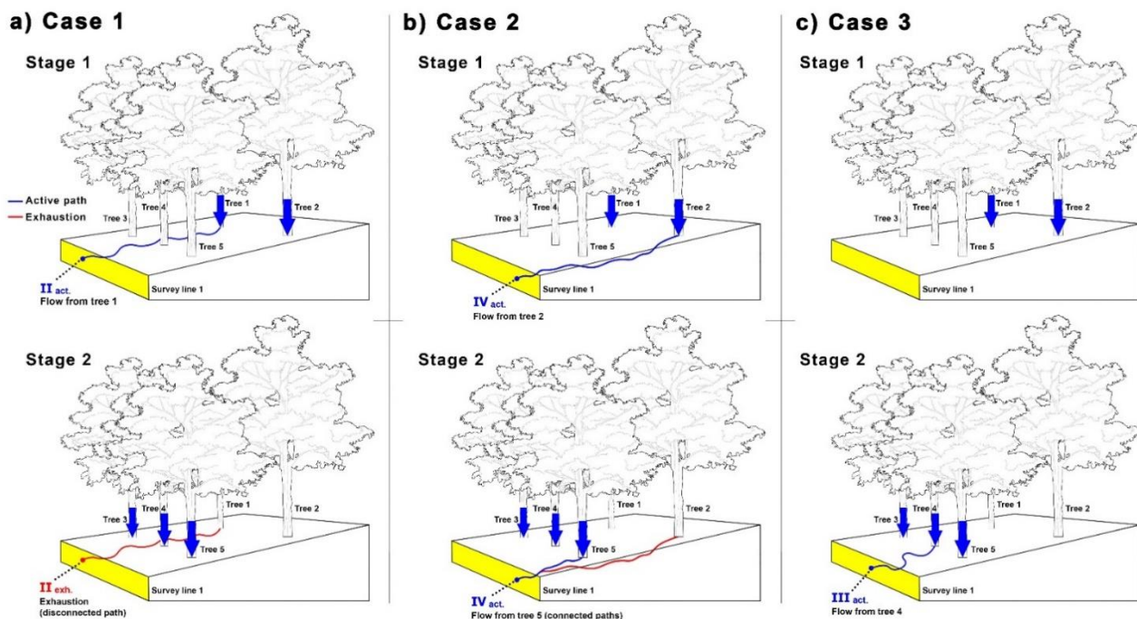
Figure 7. Graphical example of three different cases of activation of stemflow-induced preferential flow paths (a, b and c). The example depicts preferential flow paths activated during the artificial stemflow experiment, when water was poured (blue arrows) on Trees 1 and 2 (Stage 1) and then on Trees 3, 4 and 5 (Stage 2).
