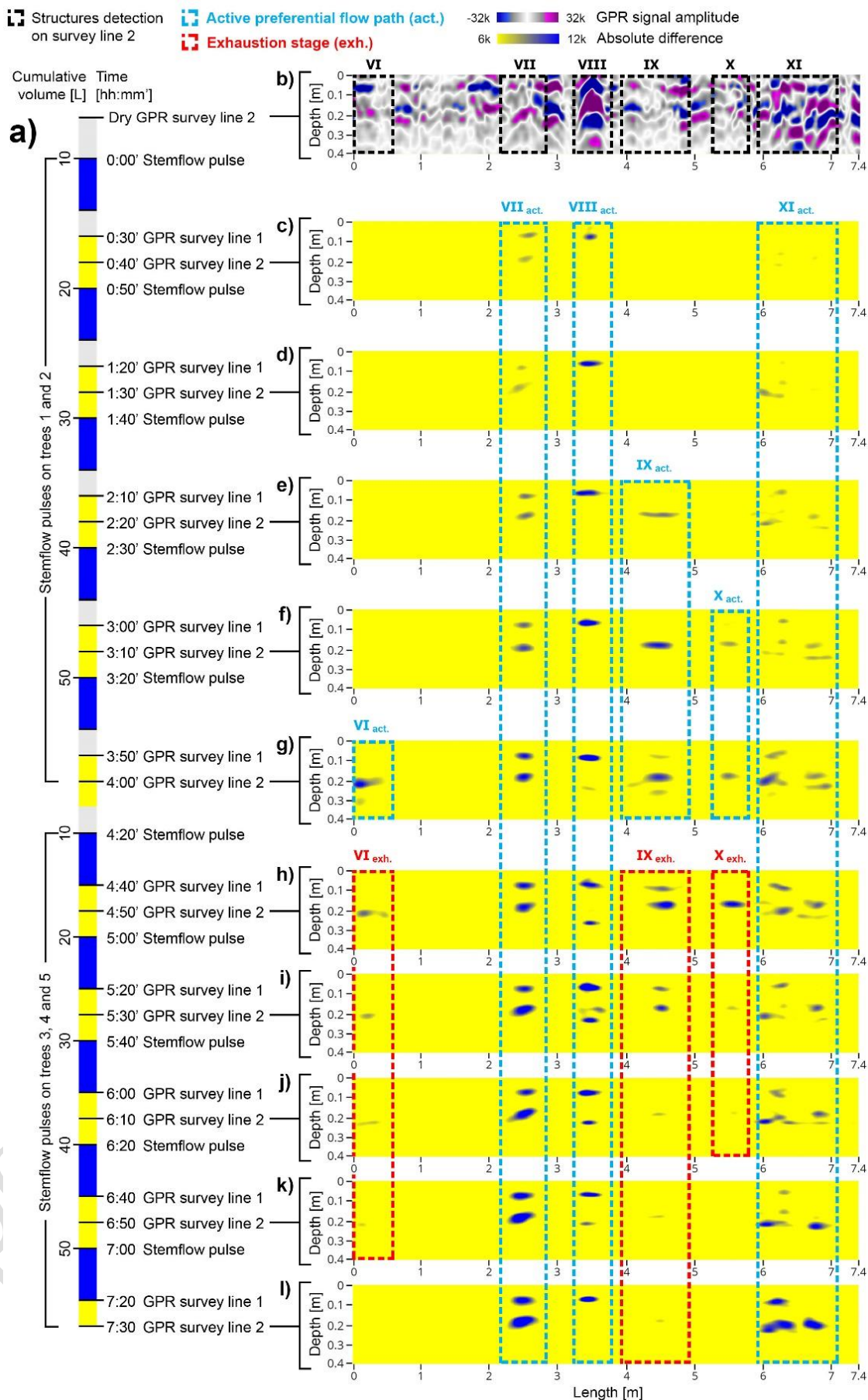
Figure 5. (a): Timeline of the repeated GPR surveys and stemflow pulses for the GPR Survey line 2. (b): Radargram collected before the execution of the artificial stemflow experiment. (c-g): Differenced radargrams obtained during the first stage of the artificial stemflow experiment, when water was poured on Trees 1 and 2. (h-l): Differenced radargrams obtained during the second stage of the artificial stemflow experiment, when water was poured on Trees 3, 4 and 5. The positions of the coarse roots that triggered preferential flow paths are indicated with Roman numerals from VI to XI and black rectangles. The positions of the detected active preferential flow paths are indicated with Roman numerals followed by the subscript act. (active) and blue rectangles. The exhaustion stages are indicated with Roman numerals followed by the subscript exh. (exhaustion) and red rectangles.
