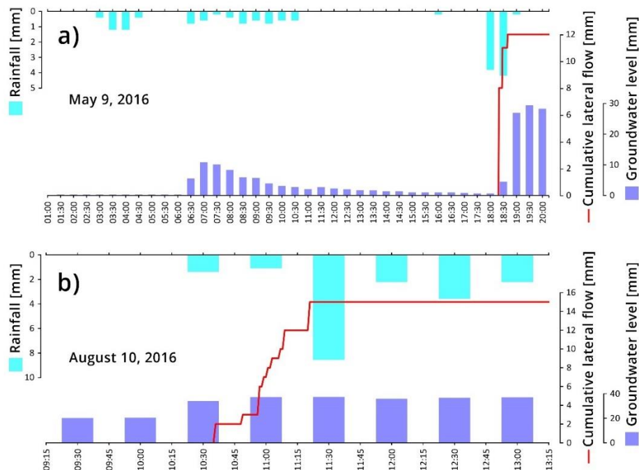
Figure 8. Data from del Campo et al. (2019) showing cumulative lateral subsurface flow collected by a trench excavated downslope from the plot to a depth of 0.4 m (the same depth was considered in this study for geophysical inspections), and groundwater levels measured on four piezometers excavated at the downslope side of the trench. These wells were aimed at checking the groundwater level and the interaction between vertical (deep drainage) and lateral flow.
