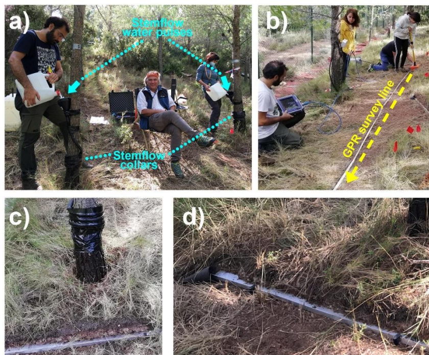
Figure 2. (a): Stemflow water pulses poured on Trees 1 and 2. (b): GPR survey carried out on Survey line 2. (c): Stemflow collar. (d): Channel for collecting overland flow.
