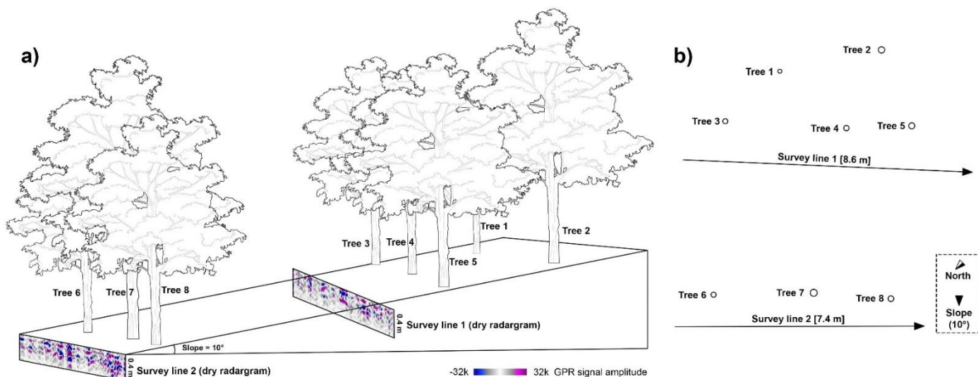
Figure 1. Experimental setup at the Calderona site. (a): Position in the studied hillslope of the GPR survey lines along with the radargrams collected before the execution of the artificial steamflow experiment. (b): Scheme of the GPR survey.
