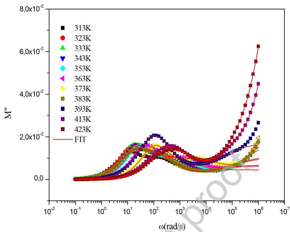
Figure 7: Variation of the imaginary part of Modulus versus frequencies of [(R)- \text{C}_5\text{H}_{14}\text{N}_2 ] \text{PdCl}_4 (1).
