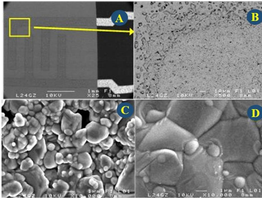
Figure 2 – FE-SEM images of \text{ZnGa}_2\text{O}_4 films grown by PLD, on Pt/alumina substrate electrodes. (A) overview of the film deposited at at 650\text{ }^\circ\text{C} and, (B) detail of intermediate region between alumina substrate and Pt electrode; (C) detail of the film covering electrodes and (D) the film in the intermediate region.
