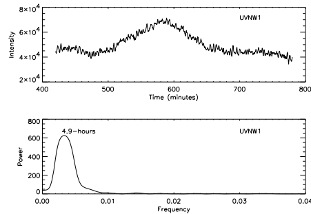
Fig. 3. Upper panel: Light curve of an isolated ultraviolet network element (UVNW1). Lower panel: Power spectra of that network element (UVNW1).
