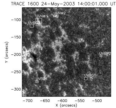
Fig. 1. One of the TRACE filtergrams obtained 2003 May 24 in the 1600 Å ultraviolet continuum, with indication of the boxes used to sample the different features, uv bright points (UVBP), uv network elements (UVNW), and uv background regions (UVBG).
