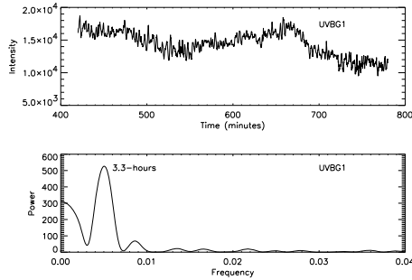
Fig. 4. Upper panel: Light curve of a background region (UVBG1). Lower panel: Power spectra of that background region (UVBG1).
