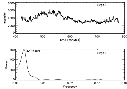
Fig. 2. Upper panel: An example of the light curve of an isolated 1600 Å continuum bright point (UVBP1) observed during 6 hours with TRACE. Lower panel: The power spectra of the light curve of that bright point (UVBP1).
