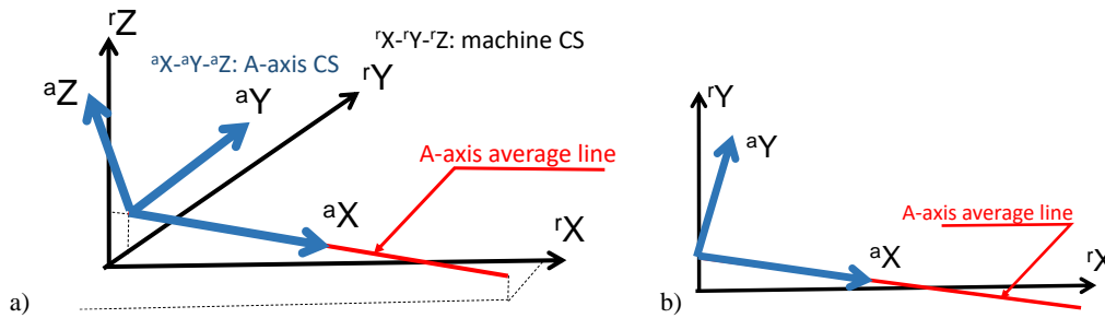
Fig. 37 Definition of the A -axis CS, when the A -axis average line is given in arbitrary position and orientation in the machine CS, a) in 3D view, b) projected onto the {}^r X - {}^r Y plane. Its {}^a X -axis is aligned to the A -axis average line. The origin is on the {}^r Y - {}^r Z plane.
