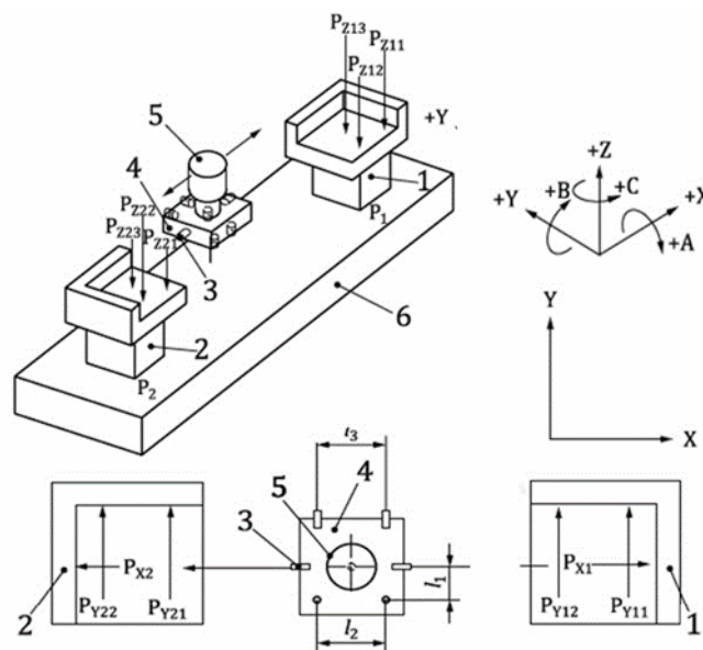
1 target right; 2 target left; 3 gap sensor; 4 sensor fixture; 5 machine spindle; 6 machine table l_1, l_2, l_3 distances between sensors used to calculate angular distortions
