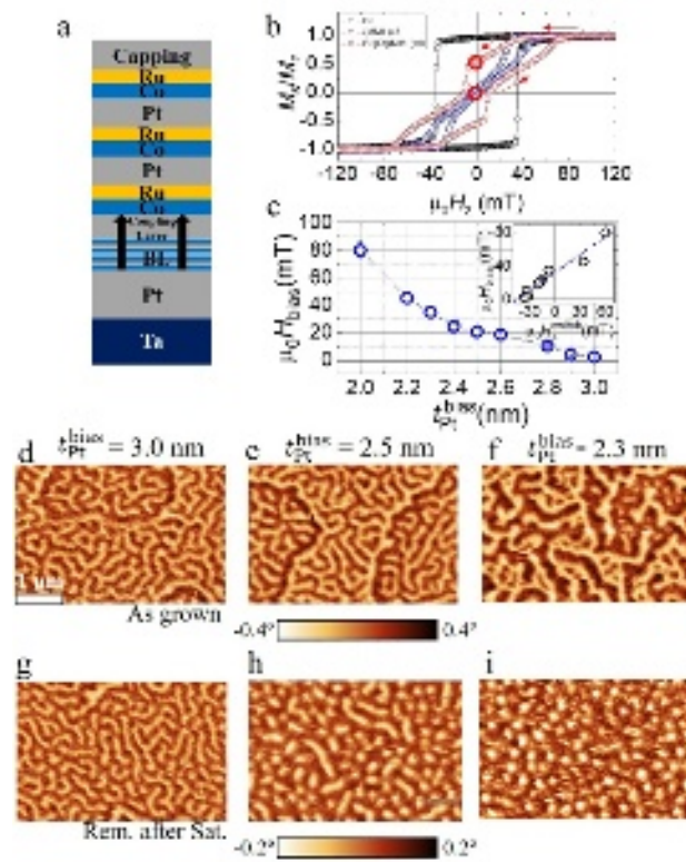
FIG. 3. a) Sketch of BL|Pt( t_{Pt} )|MML. BL is the bias-layer with stacking: (Pt(0.45)|Co(0.6)) _{\times 4} , t_{Pt} the Pt coupling-layer thickness and MML the multilayer hosting SP (Pt(8)|Co(1.6)|Ru(1.4)) _{\times 3} . b) AGFM out-of-plane hysteresis loops of BL (black), MML (blue) and BL|Pt(2.3)|MML (red). c) Effective bias field ( \mu_0 H_{bias} ) as function of Pt coupling-layer ( t_{Pt} ). The inset is \mu_0 H_{bias} vs switching field ( \mu_0 H_{switch} ). d-i) MFM images of as grown remanence after saturation state for Pt coupling-layer thickness t_{Pt}=3.0 nm (d, g), t_{Pt}=2.5 nm (e, h), t_{Pt}=2.3 nm (f, i).
