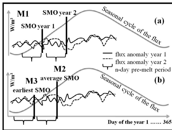
Figure 1. Schema of three methods (M1, M2 and M3) used to determine the pre-melt period and for calculation of the flux anomaly prior to SMO. In method M1 the pre-melt period is defined to start n days ( n = 1-40 ) prior to the exact local SMO date, which varies both interannually and spatially. In methods M2 and M3 the pre-melt period varies spatially but not interannually. In M2 the pre-melt period starts n days before the local 20-year average SMO date, whereas in M3 the pre-melt period starts n days before the earliest local SMO during the 20-year period. The SMO date itself is not included in the n -day pre-melt period.
