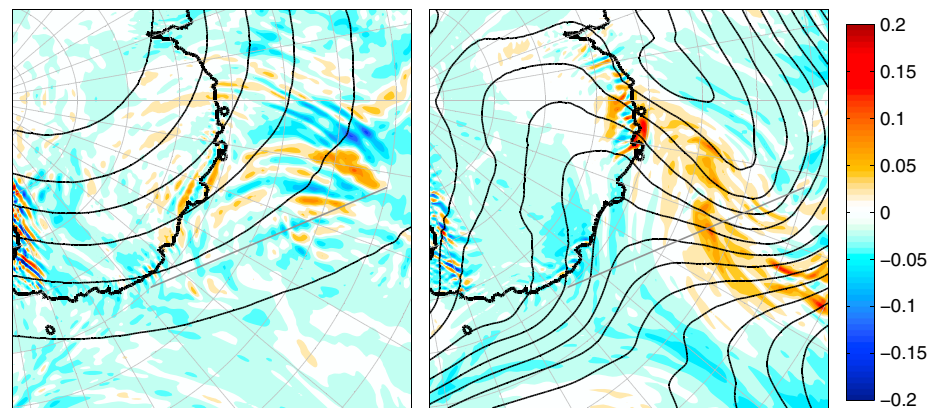
Figure 17. Vertical velocity in \text{m s}^{-1} at altitude (left) z = 20 \text{ km} and (right) z = 5 \text{ km} in the dry simulation for day 313.75, to be compared with Figure 11 (middle).
