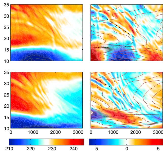
Figure 15. (left) Simulated temperature and (right) temperature perturbation (in K) with overlaid black contours of the background temperature from the WRF simulations, along the same sections as Figure 14. Horizontal and vertical coordinates are given in kilometer.
