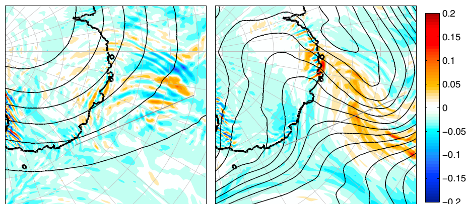
Figure 17. Vertical velocity in \text{m s}^{-1} at altitude (left) z = 20 km and (right) z = 5 km in the dry simulation for day 313.75, to be compared with Figure 11 (middle).
