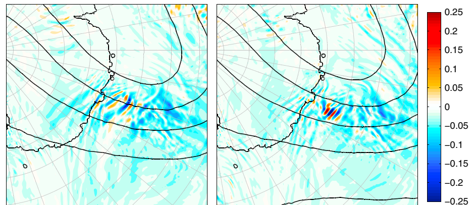
Figure A1. Vertical velocity in \text{m s}^{-1} for day 320, 00:00 UT (left) from the simulation started on day 317, 00:00 UT, and (right) from that started on day 319, 00:00 UT.
