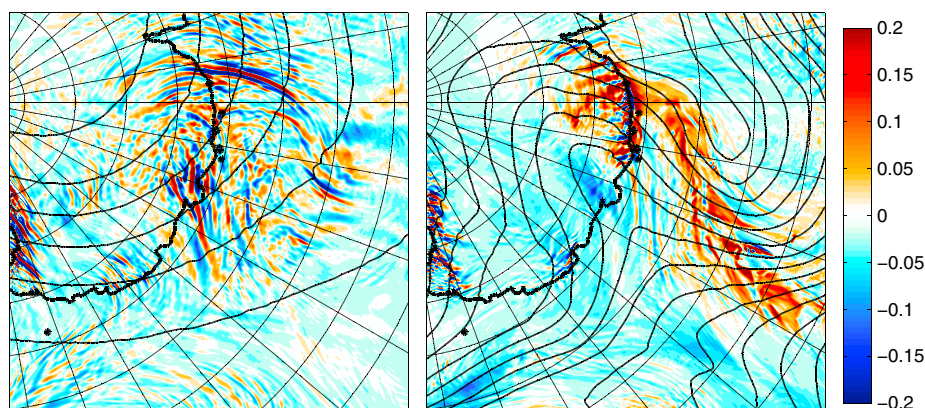
Figure 19. Simulated vertical velocity in \text{m s}^{-1} at z = 20 (left) and 5 \text{ km} from the high-resolution simulation ( \Delta x = 10 \text{ km} ), to be compared with Figure 11 (middle) (the color range is the same).
