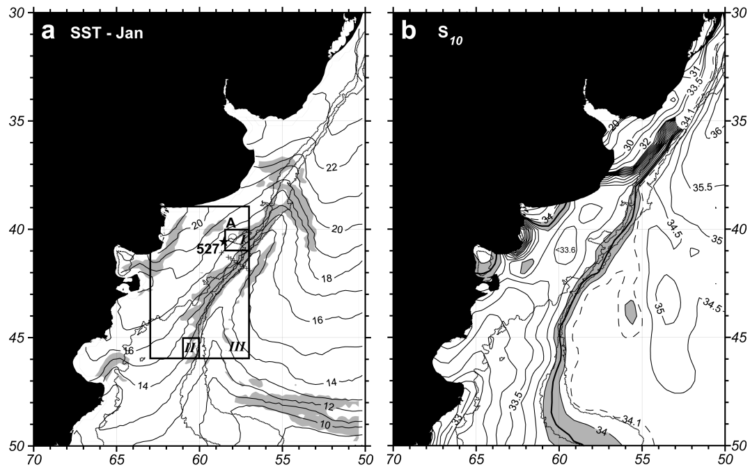
Fig. 1. (a) Mean January distribution of sea surface temperature based on 15 years of satellite data (1985–1999). Contour interval is 1\text{ }^{\circ}\text{C} . Site A is indicated by an open circle, regions I, II and III are indicated by black rectangles. Also shown are the locations of the hydrographic section shown in Fig. 2 (+), and station 527 ( \star ). (b) Climatological salinity distribution at 10 m depth. Contour intervals for S_{10} > 32.5 over the continental shelf are 0.1, and offshore 0.5 except when indicated. The grey shadings indicate the regions where the horizontal temperature gradient is larger than 0.018\text{ }^{\circ}\text{C}/\text{km} in (a) and the 10 m salinities are within the 33.8–34 range in (b). The dotted lines in both panels indicate the 100, 200 and 1000 m isobaths from GEBCO.
