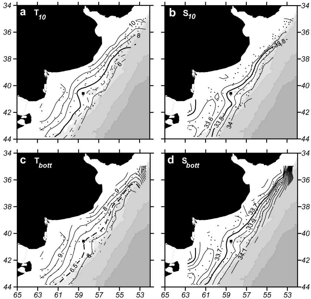
Fig. 7. Distributions of temperature ( a and c ) and salinity ( b and d ) at 10 m depth (upper panels) and bottom (lower panels), based on hydrographic data collected in July 1996. The station locations are indicated ( \bullet ), station 527 with a large square ( \blacksquare ). The background shading are the 100, 200, 1000, 3000 and 5000 m isobaths.
