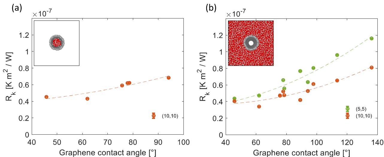
Figure 6: TBR at the inner wall-water interface for the a) (10,10) CNT, and b) at the outer wall-water interface for the (5,5) and (10,10) CNTs. Dashed lines are guides for the eye.
