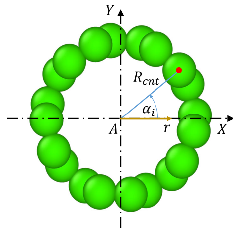
Figure 5: Cross-section of a (5,5) CNT.
