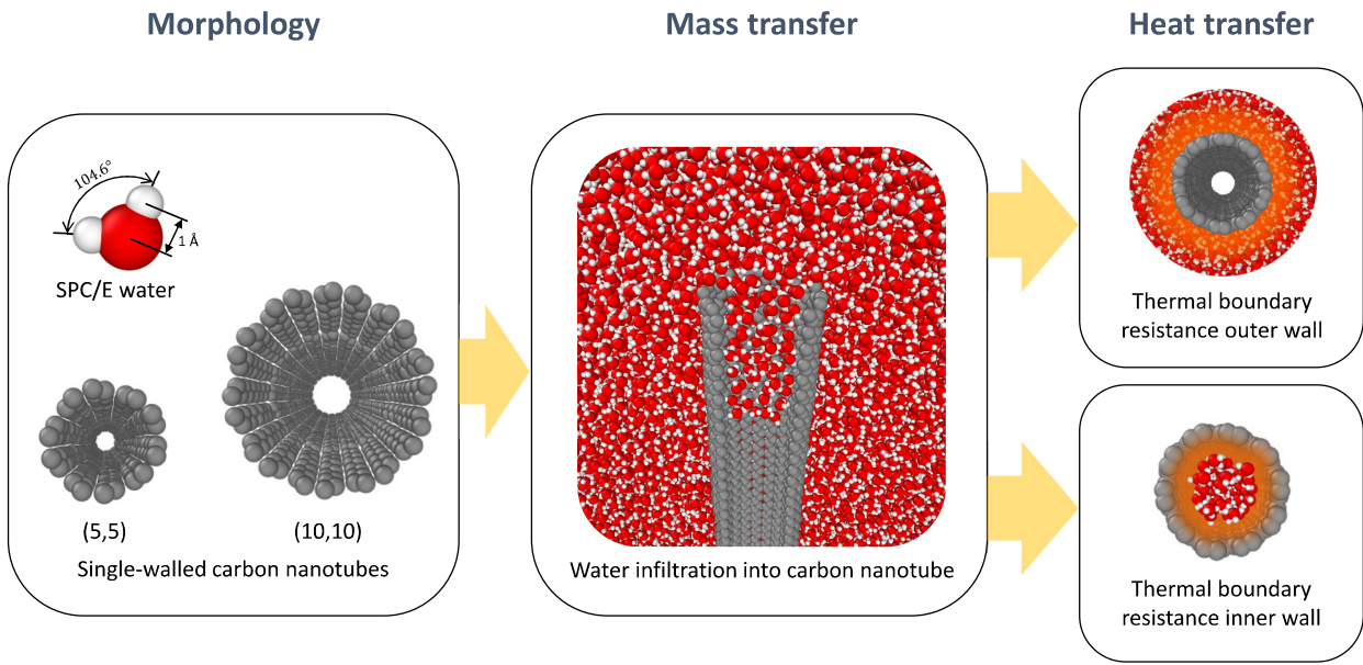
Figure 1: Pictorial representation of the simulation workflow performed. On the left, the water model adopted (SPC/E) and the two CNTs used ((5,5) and (10,10) chiral index). In the middle, a sketch of water filling of the CNTs is shown. On the right, configurations used for evaluation of the TBR at the outer and inner wall interfaces with water are shown.
