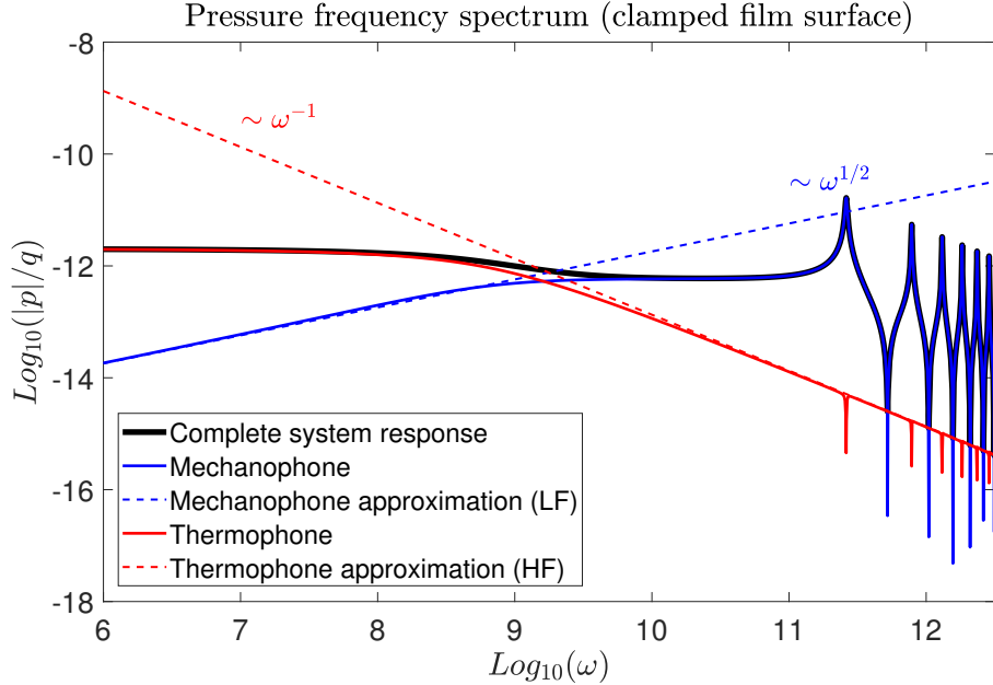
Figure 3: Water pressure intensity frequency spectrum for the case of gold clamped film surface at x = 0 ( b = -1 ) and r = 3 \times 10^{-8} \text{ m}^2\text{K/W} . The total pressure (Eq.(45), black curve) is compared to the sole mechanophone contribution (Eq.(70), blue curve) and sole thermophone contribution (Eq.(76), red curve). Moreover, the low-frequency approximation of the sole mechanophone response (Eq.(72), blue dashed line) and the high-frequency approximation of the sole thermophone response (Eq.(79), red dashed line) are reported. The intersection of the two curves from the approximations identifies the threshold frequency beyond which the mechanophone mechanism becomes predominant.
