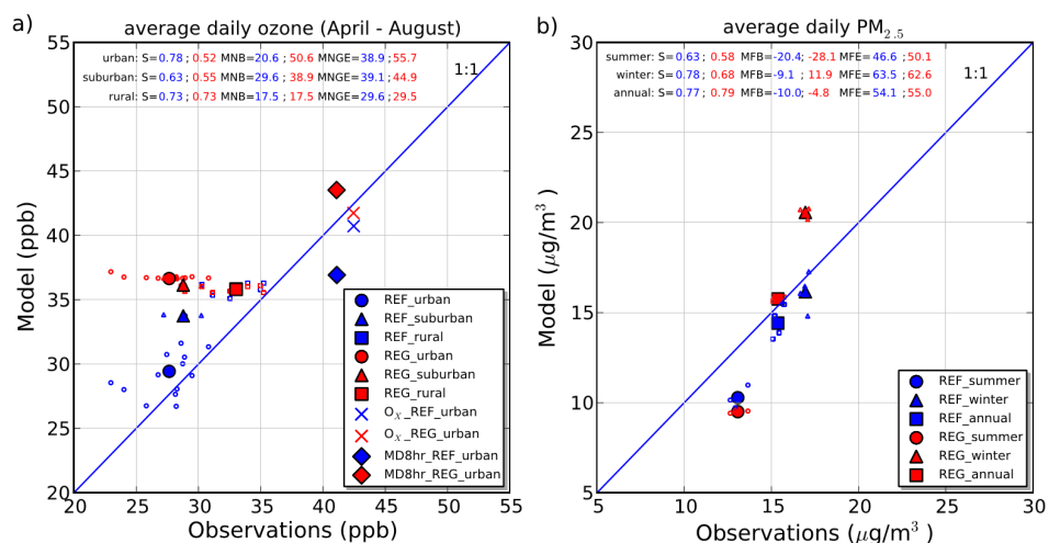
Figure 13. (a) Scatter plots of daily average ozone concentrations at urban, suburban and rural stations from the REF and REG simulations. The odd oxygen ( O_x ) and daily maximum at urban locations is also shown. (b) Daily average PM 2.5 concentrations in wintertime (DJF), summertime (JJA) and on annual basis over urban stations.
