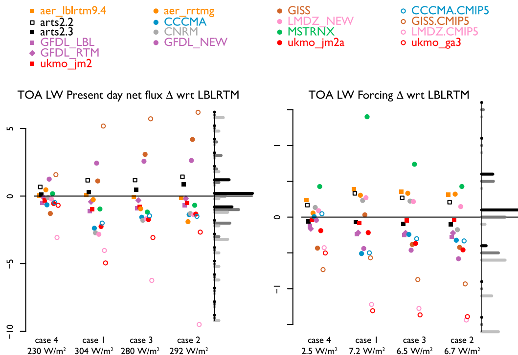
Figure 1. (left) Errors in top-of-atmosphere net downward broadband longwave flux under present-day conditions and (right) error in forcing from CO 2 concentrations quadrupled from present-day values for a variety of reference models (squares, including one high-resolution k -distribution model) and parameterizations used in climate models (circles). Calculations for four atmospheric profiles are ordered by column-integrated water vapor ranging from 0.32 to 4.85 cm. Reference values are noted. Histograms along the right edge of each panel show the error by model type (black for reference models, dark grey for current parameterizations, and light grey for parameterizations used in CMIP5; normalized across model categories) in intervals of 1 (Figure 1, left) or 0.5 (Figure 1, right) W/m 2 centered on 0. Reference models agree to within fractions of a percent in most calculations. Parameterization error is larger but still modest, with error in some parameterizations depending strongly on the water vapor path. Parameterizations that have been updated since CMIP5 are more accurate than their predecessors (compare filled circles and dark grey histogram bars to open circles and light grey bars.)
