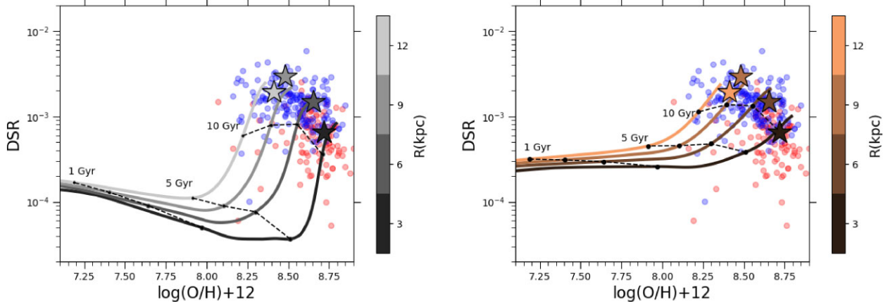
Figure 12. Dust-to-star ratio (DSR) as function of \log(\text{O}/\text{H}) + 12 for the best models at different galactocentric radii. Left panel: best model obtained assuming the Asano et al. (2013) dust accretion prescriptions (Model 5' of Table 2). The black, dark grey, grey, and light grey curves represent the evolutionary tracks at radii 3, 6, 9, and 12 kpc, respectively. Other symbols are as in Fig. 11. Right panel: best model obtained assuming the Mattsson et al. (2012) dust accretion prescriptions (Model 9' of Table 2). The dark brown, brown, light brown and orange curves represent the evolutionary tracks at radii 3, 6, 9, and 12 kpc, respectively. The other symbols and lines are as in the left panel.
