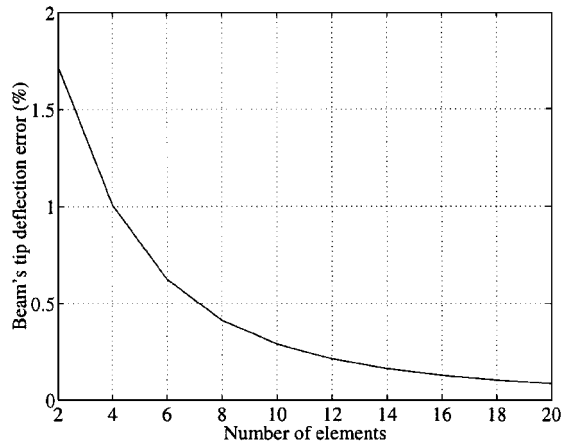
Fig. 4 Convergence of the beam's tip deflection for the shear actuation mechanism.
