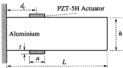
b) Extension actuation configuration
