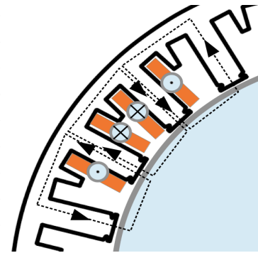
Fig. 3. Magnetic core around two consecutive coils of a CW-PMSM.
