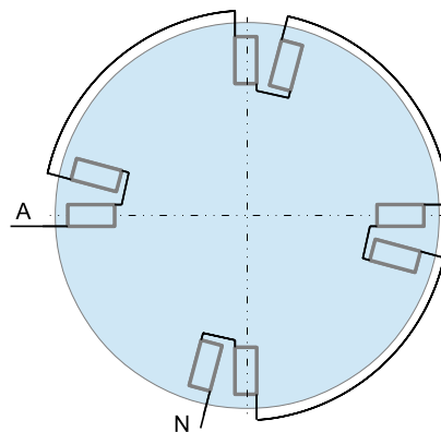
Fig. 1. Phase A of a 18 poles 24 teeth CW-PSMS made of 4 coil-pairs.
